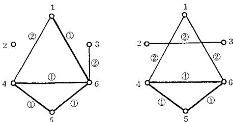
Fig. 2. Schematic digrams showing the similarity of micro environmental effects on six positions on an ear leaf. Position numbers are those of Fig. 1.
