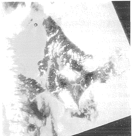
Photo 1. Visible image received: NOAA/AVHRR (Ch. 1)-4 June, 1983.
