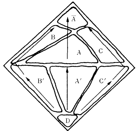
Fig. 6. Classification of peat by forming courses.
