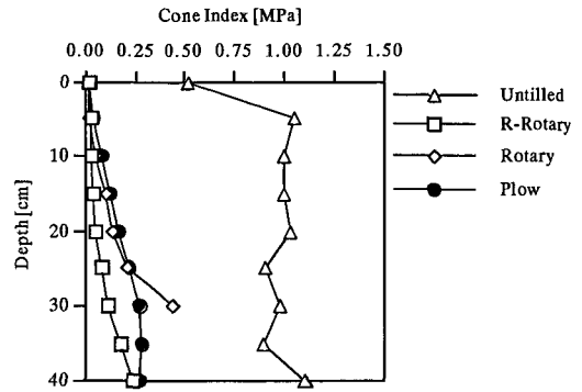
(a) Cone index of soil
