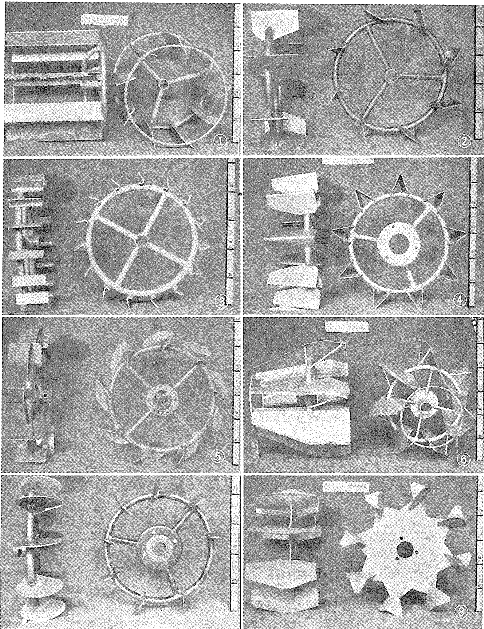
Fig. 6. Steel Wheels for Tiller (Scale...10cm)
