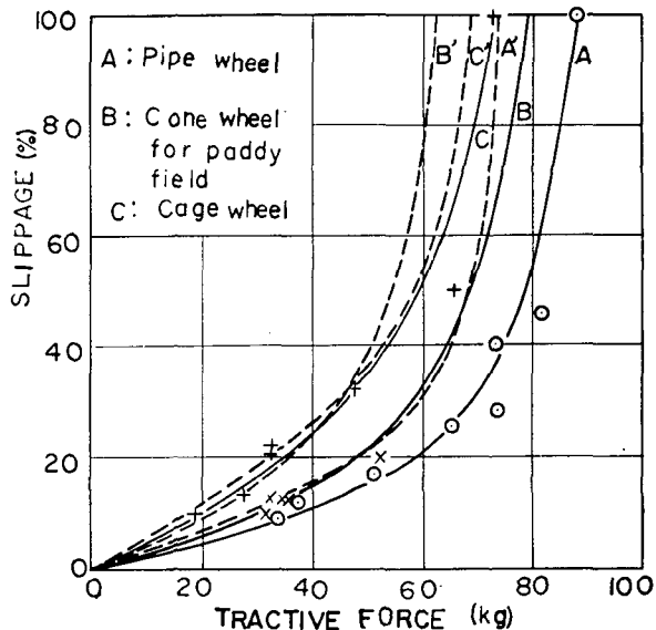
Fig. 13. Relation between tractive force and slippages of wheels for paddy field.
