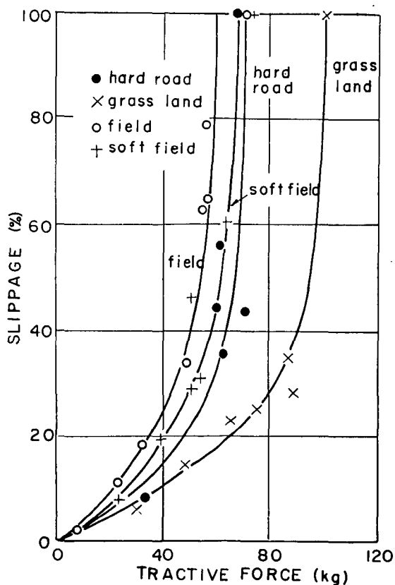
Fig. 8. Tractive force of tiller with pneumatic wheel. (Light duty tiller)
