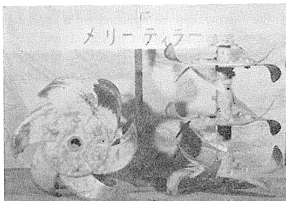
Fig. 3. Cutaway Rotor.
