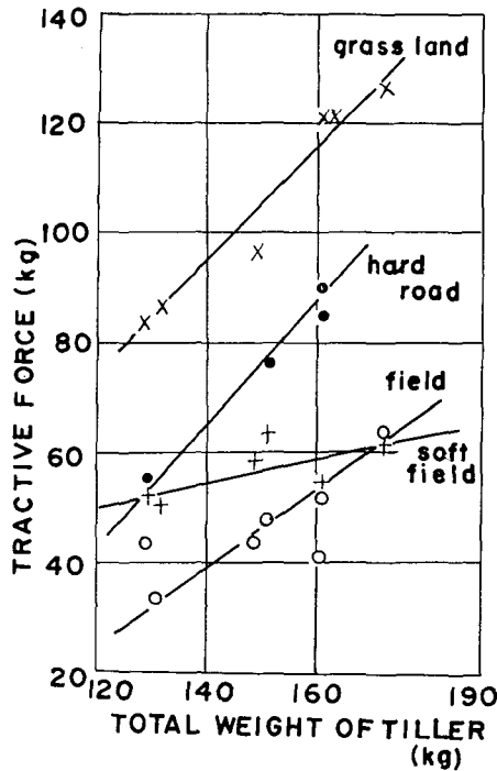
Fig. 10. Relation between tiller weight and tractive force. (at 30% slippage of wheel)
