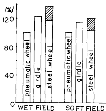
Fig. 11. Comparison of tractive force among three types of wheels.
