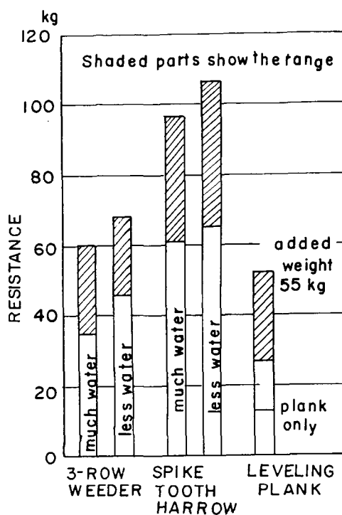
Fig. 12. Tractive resistance of some implements on paddy field.
