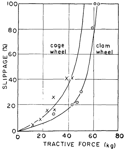
Fig. 14. Relation between tractive forces and slippages of wheels. ("Clam" wheel & Cage wheel)
