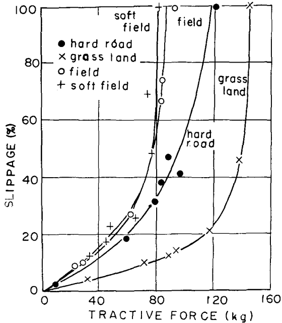
Fig. 9. Tractive force of tiller with pneumatic wheel. (Heavy duty tiller)
