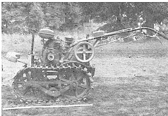
Fig. 7. Special Tiller equipped with Crawlers.
