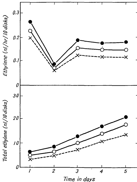
Figure 2. Time course experiment of ethylene evolution of excised tissues derived from various parts of tuber. —●— = apex, —○— = cortex, - - x - - = pith.
