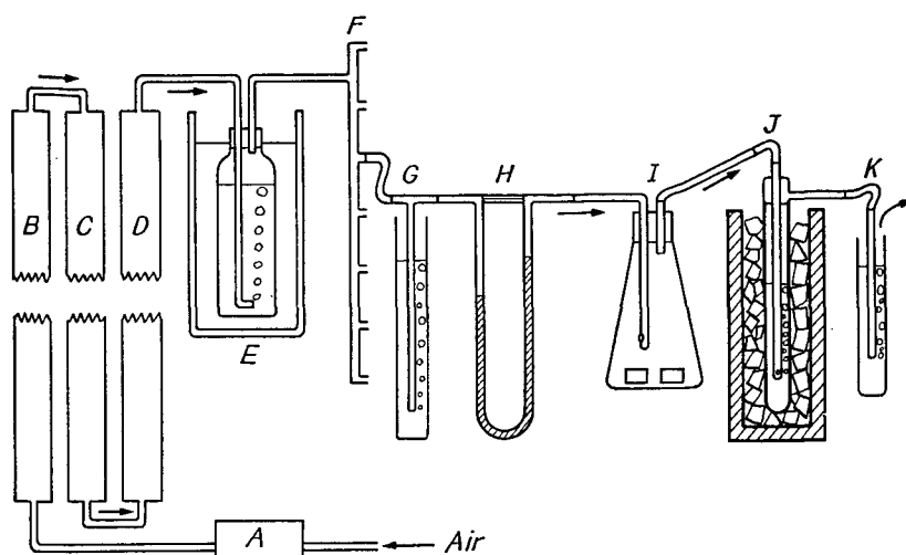
Figure 1. Trapping apparatus of ethylene evolved by potato tubers and tissues. A=air pressure pump. B=column tightly packed with absorbent cotton. C=column filled with active charcoal. D=column filled with \text{KMnO}_4 adsorbed silica gel. E=bubbling tower maintained at 25^\circ\text{C} water bath. F=manifold. G=barostat tower. H=air flow meter. I=container. J=ethylene trapping tube with mercuric perchlorate solution maintained at 0^\circ\text{C} by ice. K=back pressure tower. Spiral glass in the water bath as described in the methods is omitted here.
