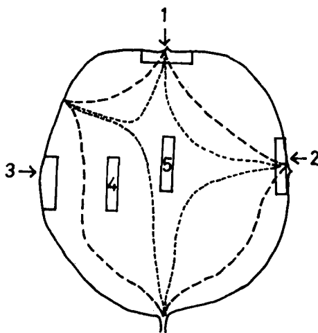
Fig. 1. Representative portions of potato tuber tissues selected for analysis of IAA metabolism. Disc-shaped tissues, 5 mm in diameter and 2 mm in thickness, were excised from different parts of tuber which were designated as apical bud (1), lateral bud (2), cortex (3), perimedullary pith (4) and central pith (5), respectively.
