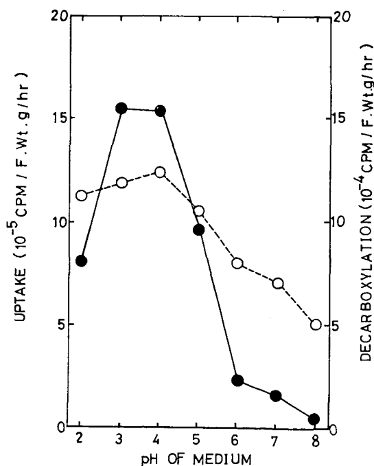
Fig. 2. Comparison of uptake (—●—) and decarboxylation (···○···) of IAA-1- ^{14}\text{C} by the potato tuber tissues incubated at various values of pH for 2 hr.
