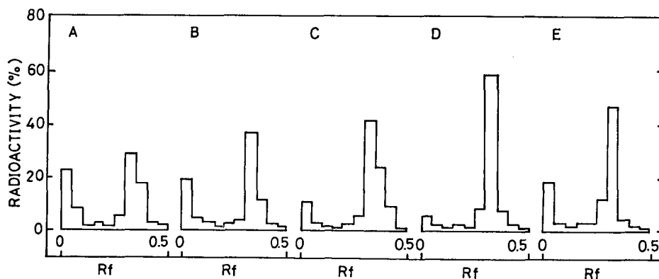
Fig. 4. Paper chromatograms of the ethanol extracts of tissues incubated with IAA-1- ^{14} C. Tissues of potato tuber were obtained from apical bud (A), lateral bud (B), cortex (C), perimedullary pith (D) and central pith (E), respectively. Extracts prepared from those tissues were chromatographed on paper developed with iso-propanol: 28% ammonia: water (10:1:1; v/v/v). The radioactive regions with Rf of 0.01 and 0.3 are IAA-conjugate and IAA, respectively. There were no other radioactive regions on the the chromatogams.
