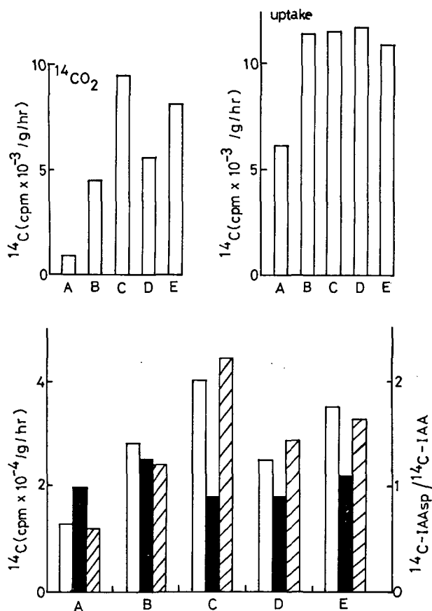
Fig. 6. Effect of air ventilation with and without ethylene on the IAA metabolism of tissue discs of potato tuber. A=control, B=air ventilation without ethylene, C=air ventilation with ethylene for first 2 days, D=air ventilation with ethylene for later 2 days, E=air ventilation with ethylene throughout the experimental period. Upper: Comparison of decarboxylation (left) and uptake (right) of ^{14}\text{C} -IAA. Lower: Comparison of ^{14}\text{C} -IAA (black bar) and ^{14}\text{C} -IAA sp (white bar) of the ethanol extracts, and the ratio of ^{14}\text{C} -IAA sp to ^{14}\text{C} -IAA (hatched bar).
