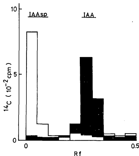
Fig. 5. Distribution of radioactivities on the chromatograms, which shows comparison between IAA conjugate fractions of being subjected by acid hydrolysis (black bar) and control (white bar). Details of procedure is represented in the text.
