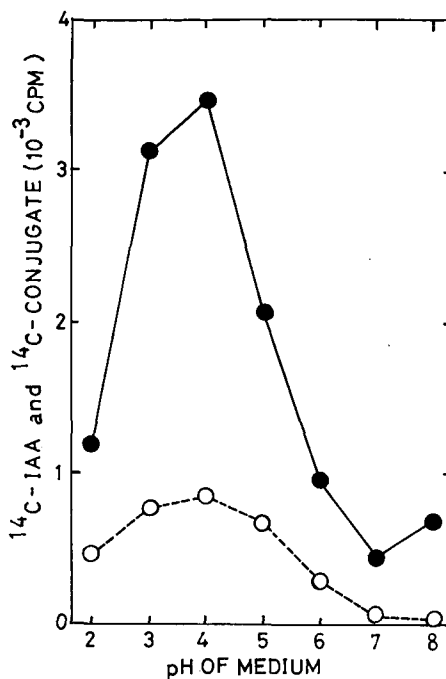
Fig. 3. Effect of different pH values of the incubation medium on the levels of free ^{14}\text{C} -IAA (—●—) and ^{14}\text{C} -conjugate (···○···) in the potato tissues incubated for 2 hr.
