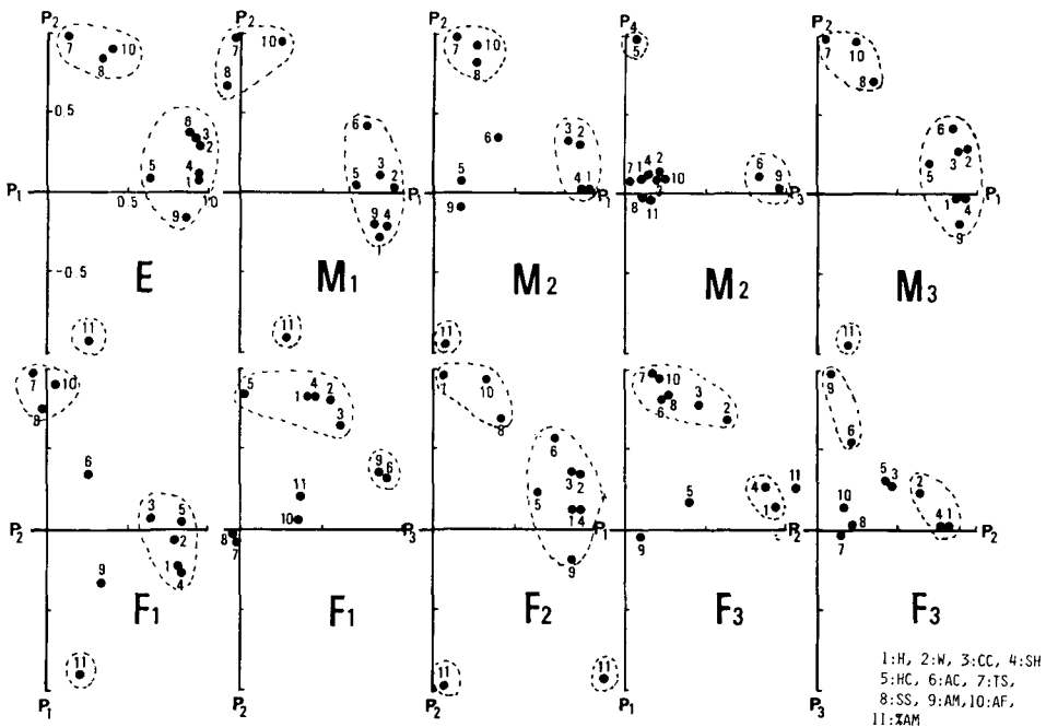
Fig. 3. Rotated components loadings (Varimax solution) on nutrient intake of Hokkaido orphanage children in 1976. Only loadings whose values were greater than an arbitrary cutoff of 0.5 were grouped by broken line.
