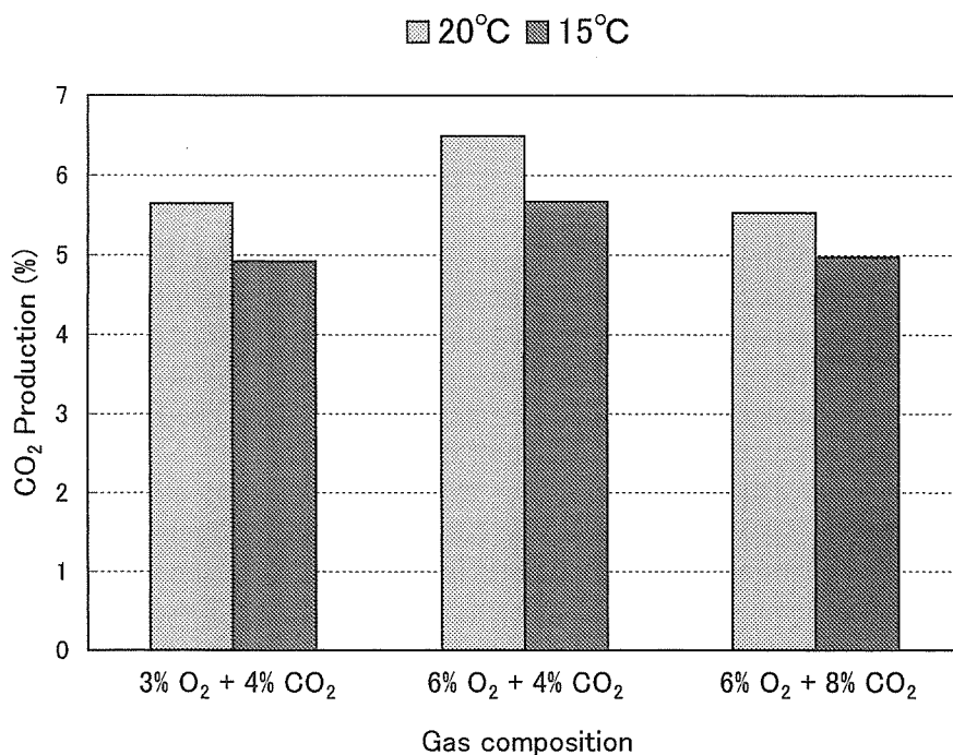
Fig. 1. The average CO 2 production in the storage chambers during the 2-day intervals.
