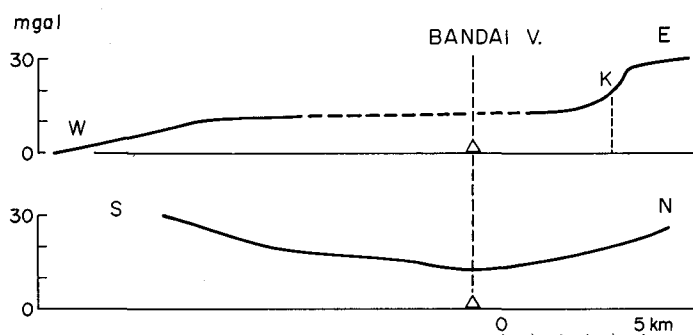
Fig. 5 Gravity anomaly profiles passing the summit of Bandai volcano in the EW and NS directions. K represents a fault.
