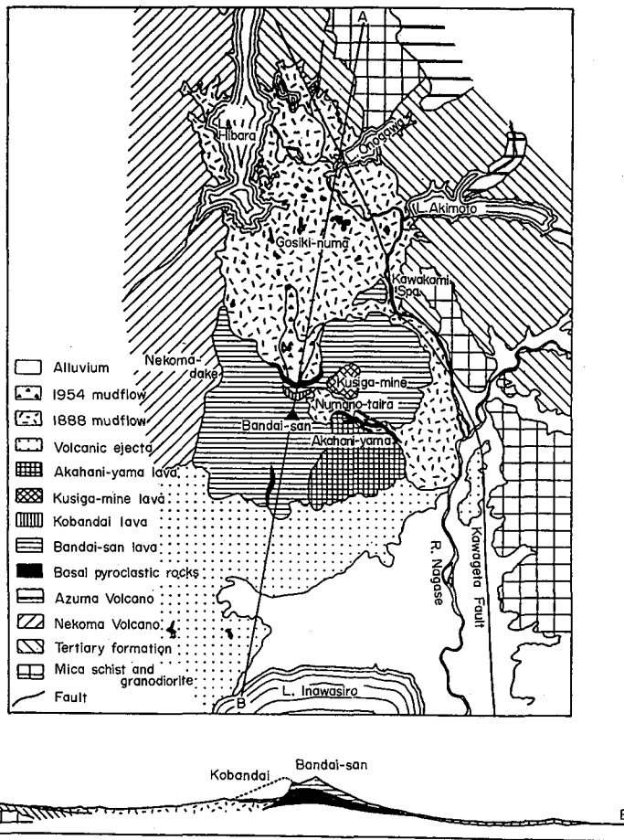
Fig. 6 Geological map of Bandai volcano (Okada, 1952)
