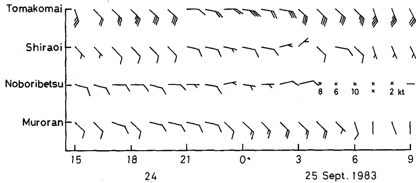
Fig. 12. Time variation of winds at AMeDAS observation points in the seaside area of the Iburi District.
