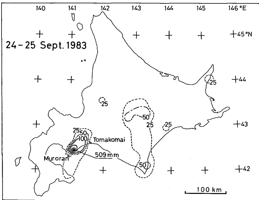
Fig. 3. Distribution of rainfall amount from 24 to 25 September 1983.
