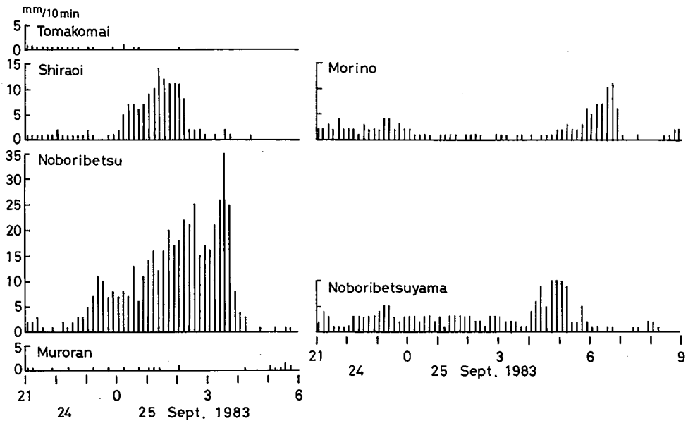
Fig. 10. Time variation of 10 minute rainfall intensity at AMeDAS observation points in the Iburi District.
