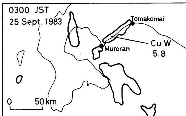
Fig. 5. Radar echo sketch by Hakodate radar on 0300 JST 25 September 1983.
