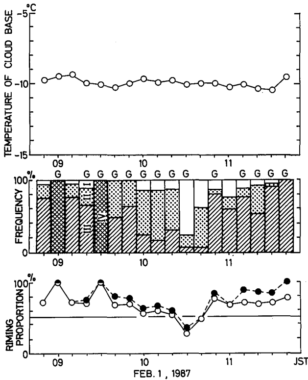
Fig. 5. Time changes of the temperature of cloud base over the observation site, frequency of snow crystals in each type and riming proportion at the observation site on 0850–1140 JST 1 February 1987. Solid circles in the lower part indicate the riming proportion incorporating the effect of graupel particles.
