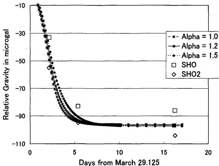
Fig. 5. Relative gravity variation at SHO (Showashinzan). Gravity changes due to uplift of mountain body are also calculated from the results in Figs. 3 and 4.
