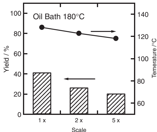
Figure 4. The yields of 4-methyl-2,3-dihydro-1 H -1,5-benzodiazepin-2-one by the reaction of 1,2-phenylenediamine and ethyl acetoacetate and the temperatures just after the reaction in different scales. The heating times are 2 min.
