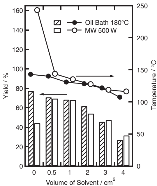
Figure 3. The yield of 4-methyl-2,3-dihydro-1 H -1,5-benzodiazepin-2-one by the reaction of 1,2-phenylenediamine and ethyl acetoacetate and the temperatures just after the reactions in different volume of the solvent of xylene. The heating times are 10 min.
