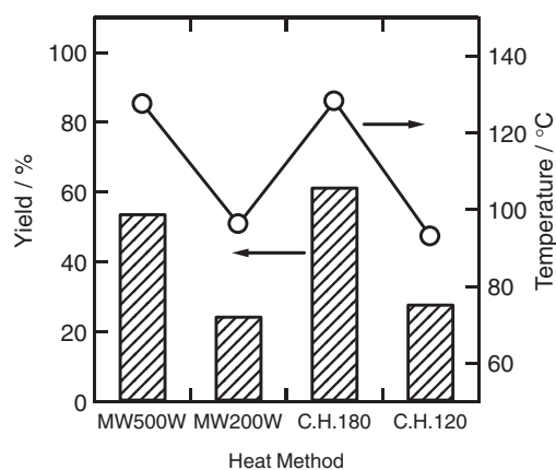
Figure 1. The yields of 4-methyl-2,3-dihydro-1 H -1,5-benzodiazepin-2-one by the reaction of 1,2-phenylenediamine and ethyl acetoacetate and the temperatures just after the reaction heated for 10 min by 500-W (MW500 W), 200-W (MW200 W) microwave irradiation, and 180-°C (C.H.180) and 120-°C (C.H.120) oil baths.
