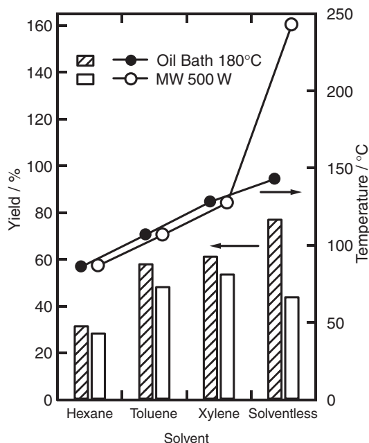
Figure 2. The yields of 4-methyl-2,3-dihydro-1 H -1,5-benzodiazepin-2-one by the reaction of 1,2-phenylenediamine and ethyl acetoacetate and the temperatures just after the reactions in different solvents. The heating times are 10 min.
