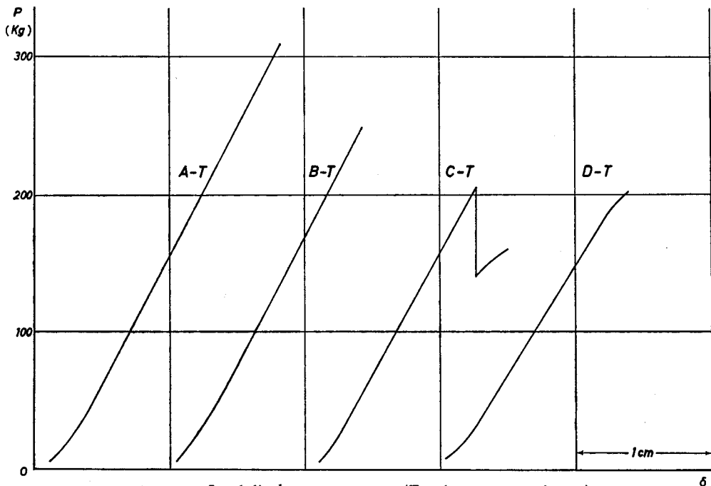
Fig. 2. Load-displacement curves (Tension type specimens).
