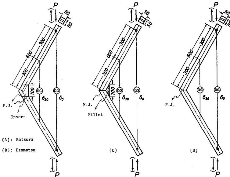
Fig. 1. Diagrams of test specimens and testing method.
