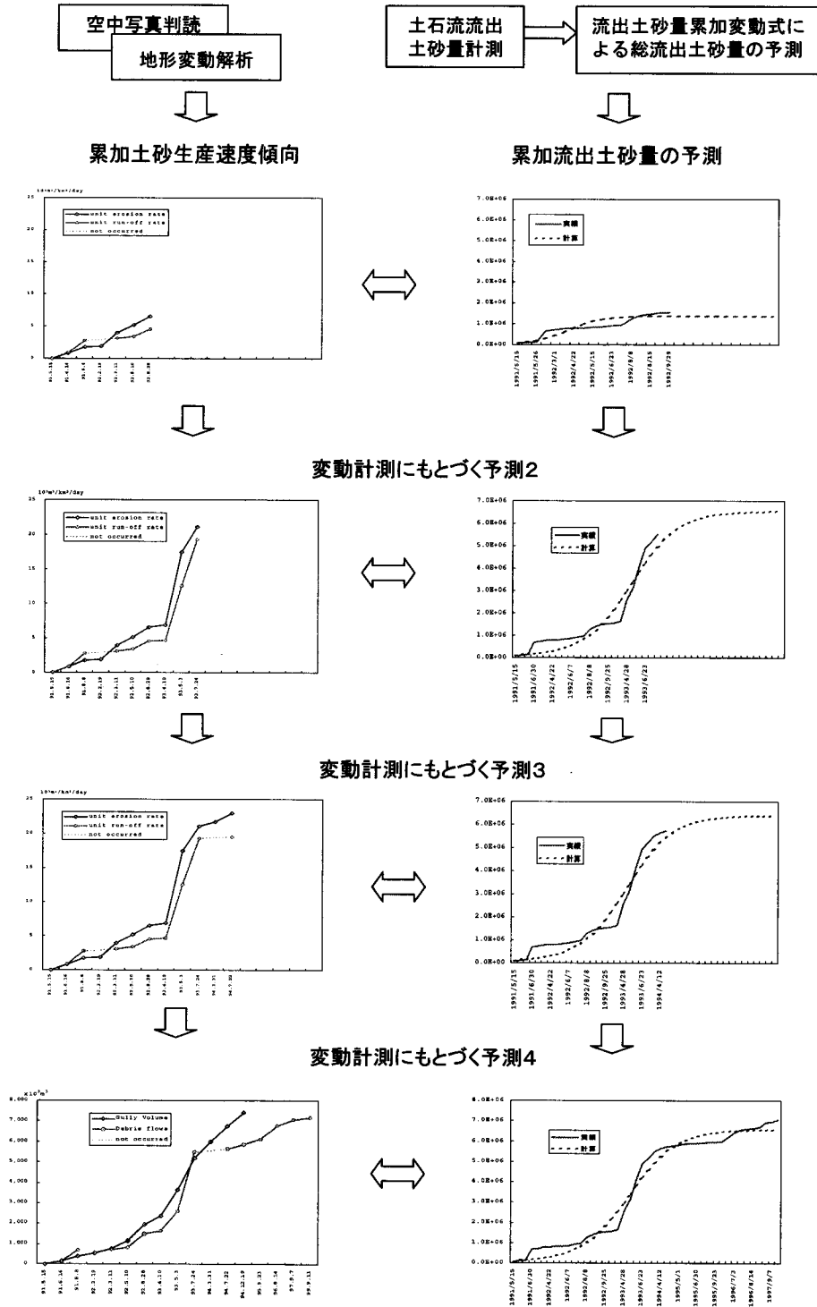
図-5.10 地形変動解析と流出土砂量累加変動式による土砂流出予測 Figure 5.10 Predicting scheme by geomorphic analysis and equation for trend of accumulated sediment discharge volume
