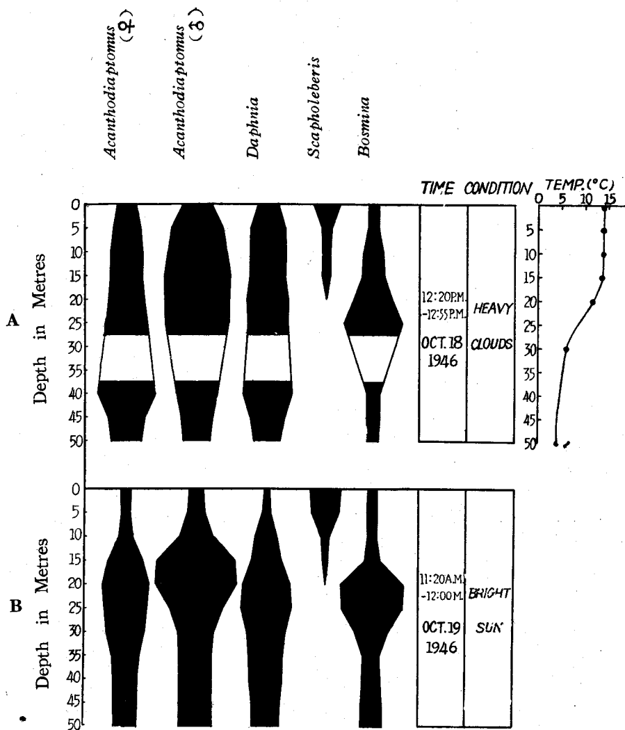
Fig. 3. Vertical distribution of plankton crustaceans in daytime in October, 1946, in the deep water of Lake Shikotsu (Observation 3) (A) Under heavy clouds on Oct. 18th (B) Under bright sun on Oct. 19th
