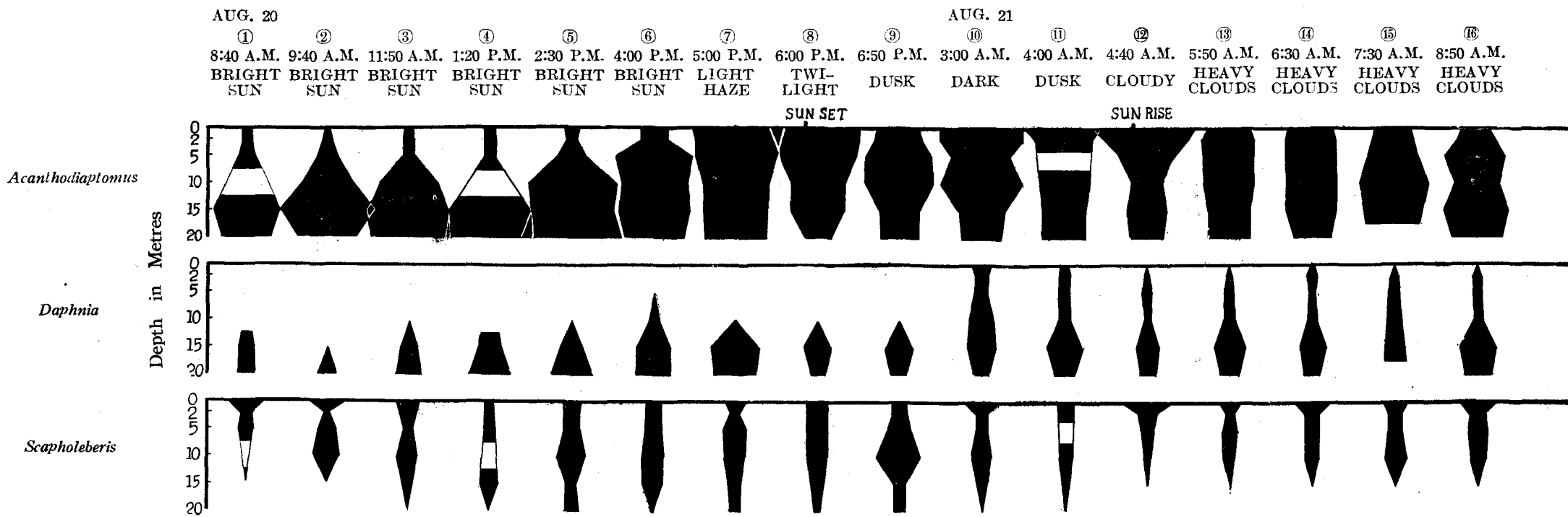
Fig. 4. Diurnal migration of plankton crustaceans in August 20th—21st, 1942, in Lake Shikotsu (Observation 4)
