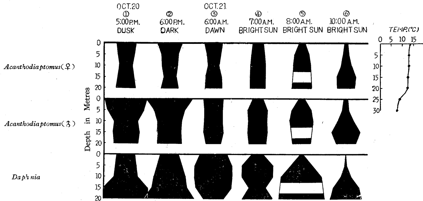
Fig. 8. Diurnal migration of plankton crustaceans in October, 1944, in Lake Shikotsu (Observation 8)
