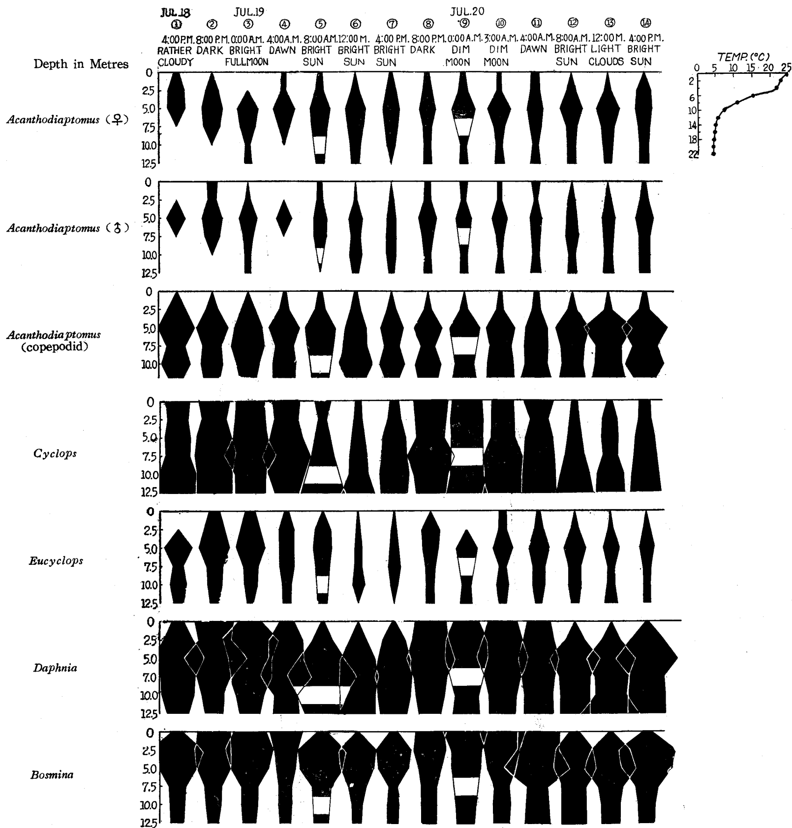
Fig. 9. Diurnal migration of plankton crustaceans in July 18th-20th, 1943, in Lake Tsugarujuni (Observation 9)
