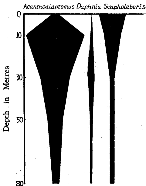
Fig. 1. Vertical distribution of plankton crustaceans at 10:30 a. m. on August 20th, 1942, under bright sun in the deep water of Lake Shikotsu (Observation 1)
