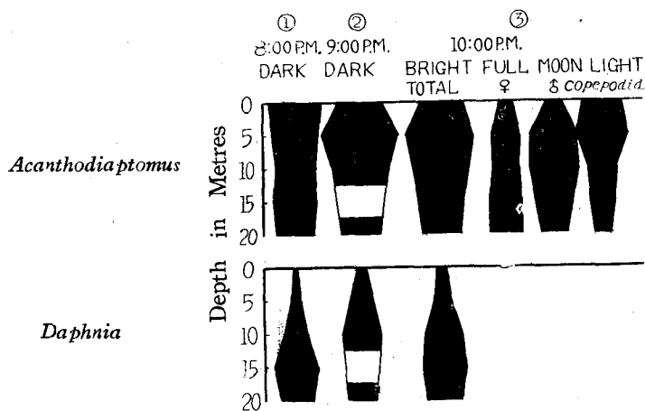
Fig. 5. Vertical distribution of plankton crustaceans at night on August 14th, 1943, in Lake Shikotsu (Observation 5)
