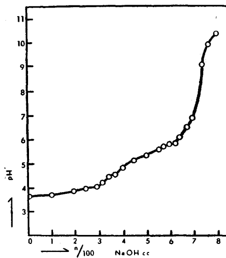
Fig. 12. Titration curve of saturated alginic acid solution "A", with n/100 NaOH
