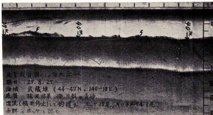
Fig. 17 Echo-image of the sea-bottom near shallowest part of the Musashi Bank when angle fishing test was made
