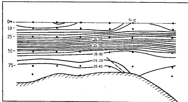
Fig. 5. Vertical profile of density in a section running from the interior (left side) toward the exterior (right side) of the Bay on September 13 and 14, 1951. St. C shows the current measurements station
