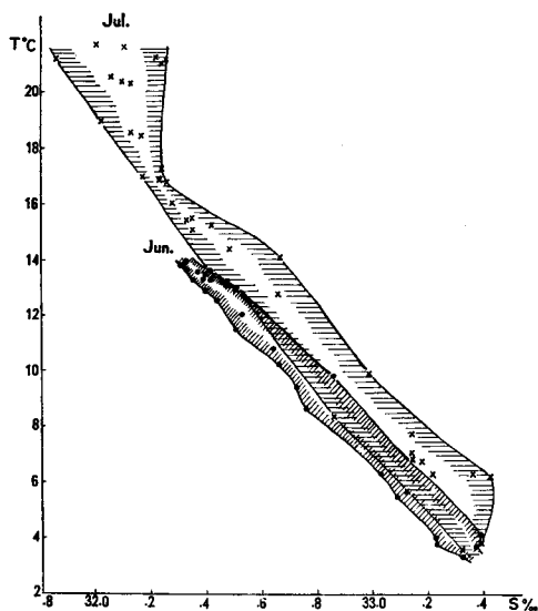
Fig. 7. Temperature-salinity relations for all stations in the Bay in June and July, 1951
