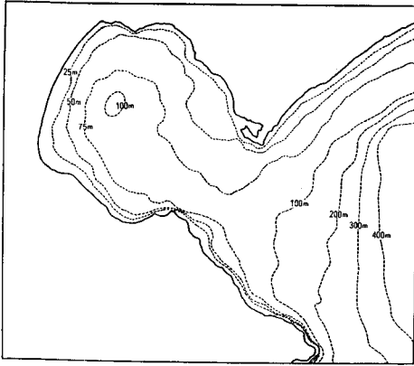
Fig. 1. Bottom contours in Funka Bay and vicinity
