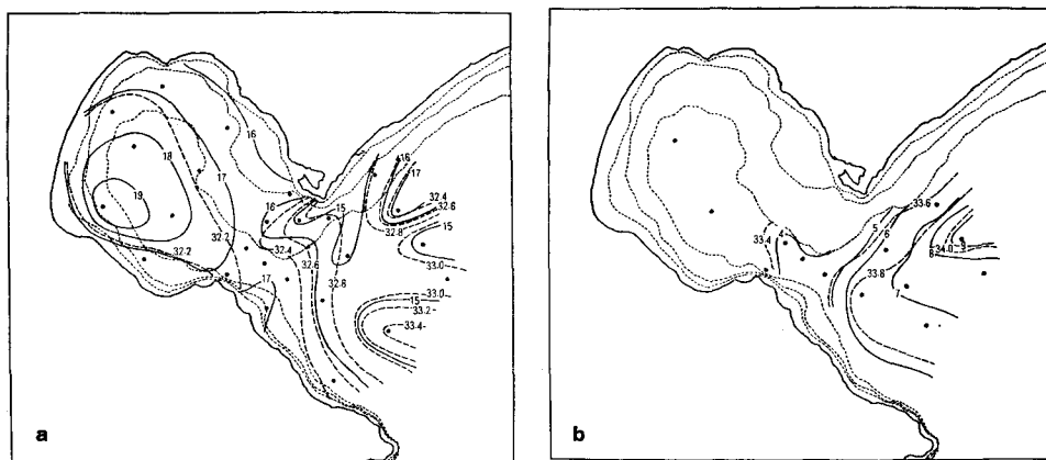
Fig. 4. Horizontal distribution of temperature and salinity on July 26 to 28, 1951 a: 10 m level b: 75 m level
