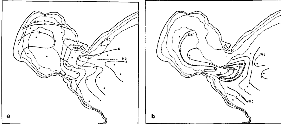
Fig. 9. Horizontal distribution of temperature and salinity on October 10 to 12, 1951 a: 10 m level b: 75 m level
