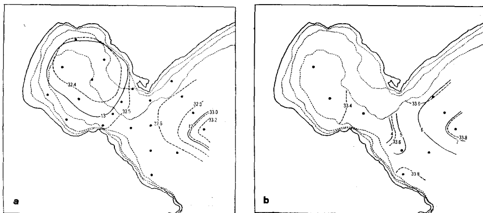
Fig. 3. Horizontal distribution of temperature and salinity on June 21 to 23, 1951 a: 10 m level b: 75 m level
