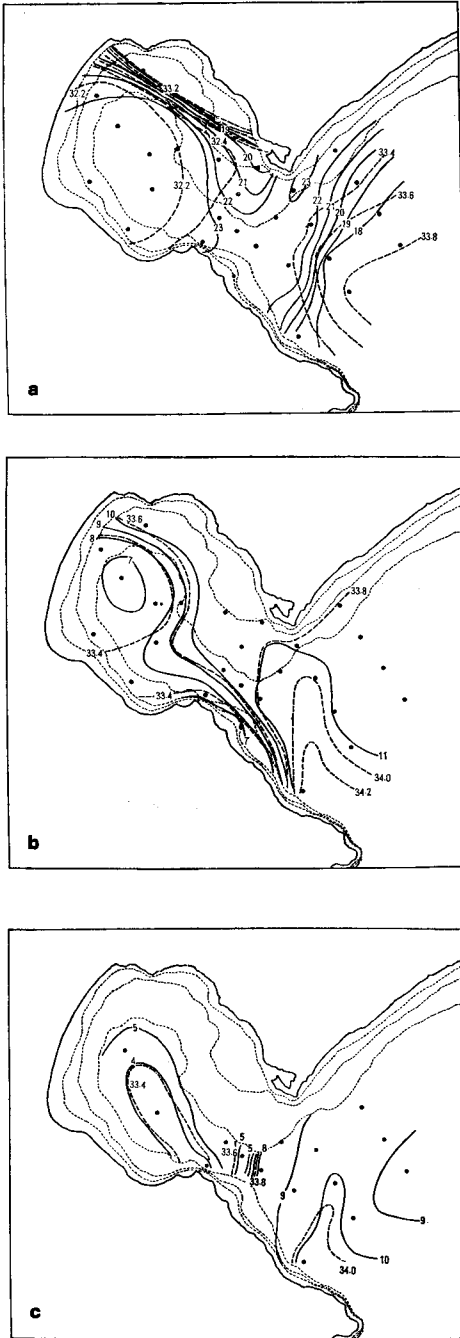
Fig. 8. Horizontal distribution of temperature and salinity on August 27 to 29, 1951 a: 10 m level b: 50 m level c: 75 m level
