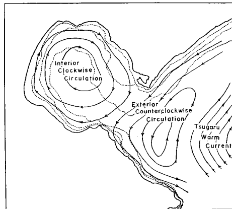
Fig. 2. Schematic representation of the current system in Funka Bay and vicinity
