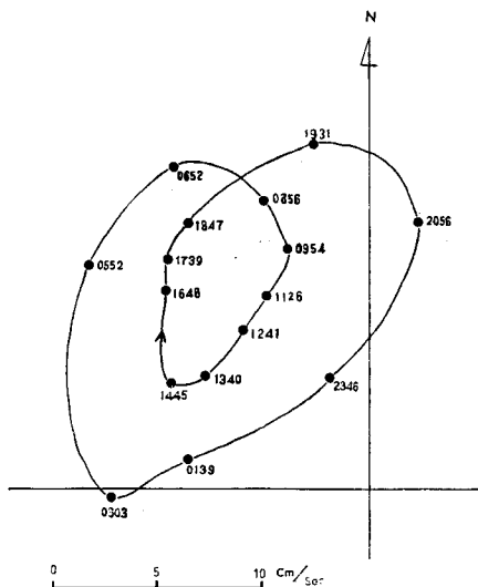
Fig. 6. Observed currents at a depth of 75 m at St. C (see Fig. 5) on September 13 and 14, 1952
