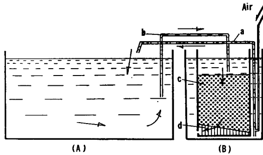
Figure 2. Diagrammatic illustration of rearing aquarium with a recirculating sea water system. (A): Aquarium, (B): Filtering chamber, a: Air lift, b: Siphon, c: Sea sand, d: Glass wool. The arrows indicate the circulation of rearing sea water.
