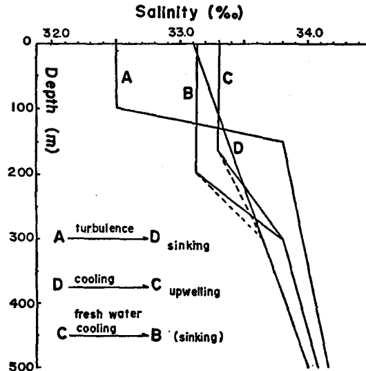
Fig. 24. Schematic representation of transformation from Type A through Type D to Type C and Type B.
