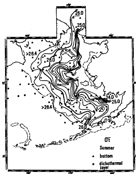
Fig. 44. Distribution of \sigma_t at the bottom of the shelf and of the dichothermal water in the basin.
