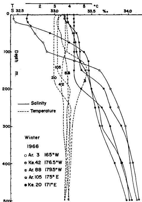
Fig. 8. Vertical distribution of temperature and salinity along the center of the Alaskan Stream in winter.
