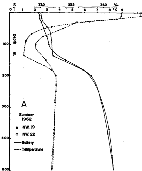
Fig. 18. Salinity and temperature curves of Type A in summer.
