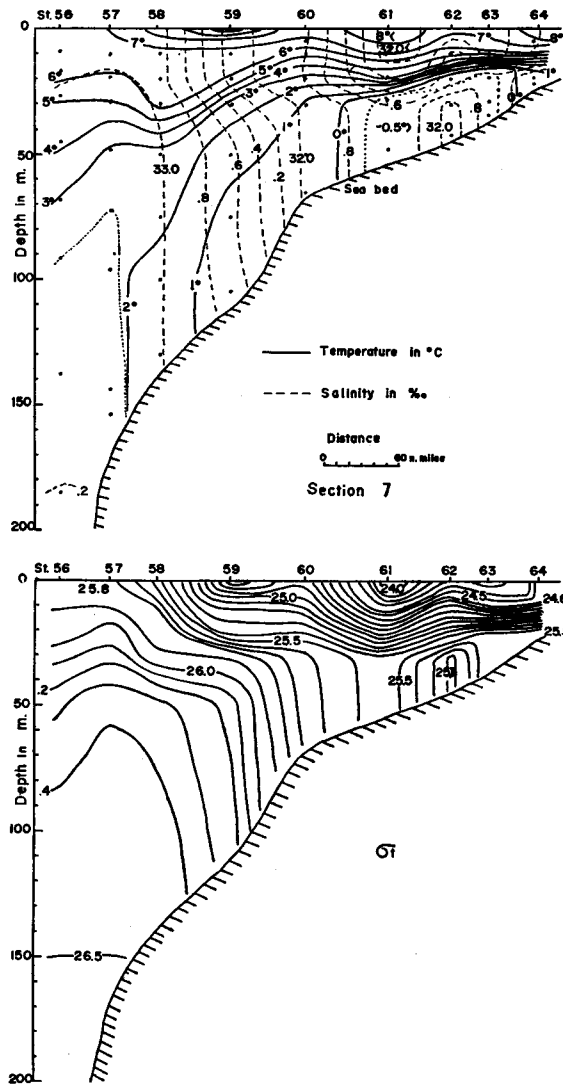
Fig. 34. Vertical sections of temperature, salinity and \sigma_t in the northern part of the shelf.
