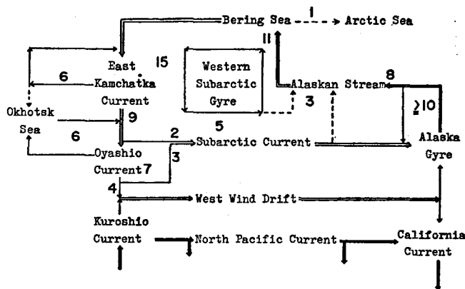
Fig. 3. Schematic diagram of relative transport in the northern North Pacific Ocean in winter. Numerals indicate volume transport ( \times 10^6 m 3 /sec) in reference to the 1,000-m. level.
