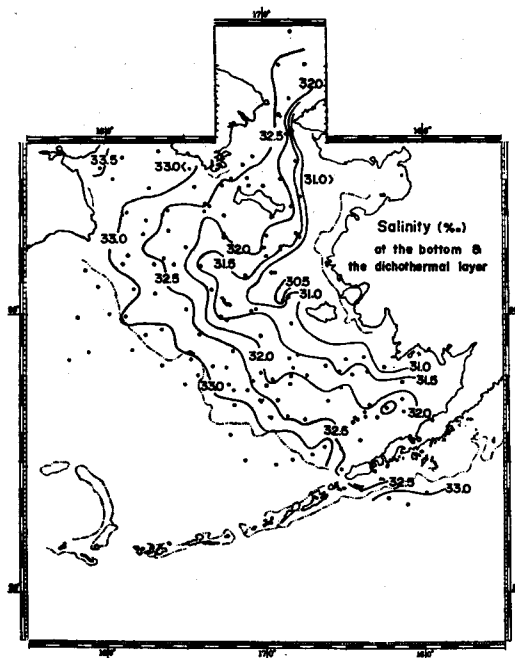
Fig. 27. Salinity distribution at the bottom on the shelf in summer.
