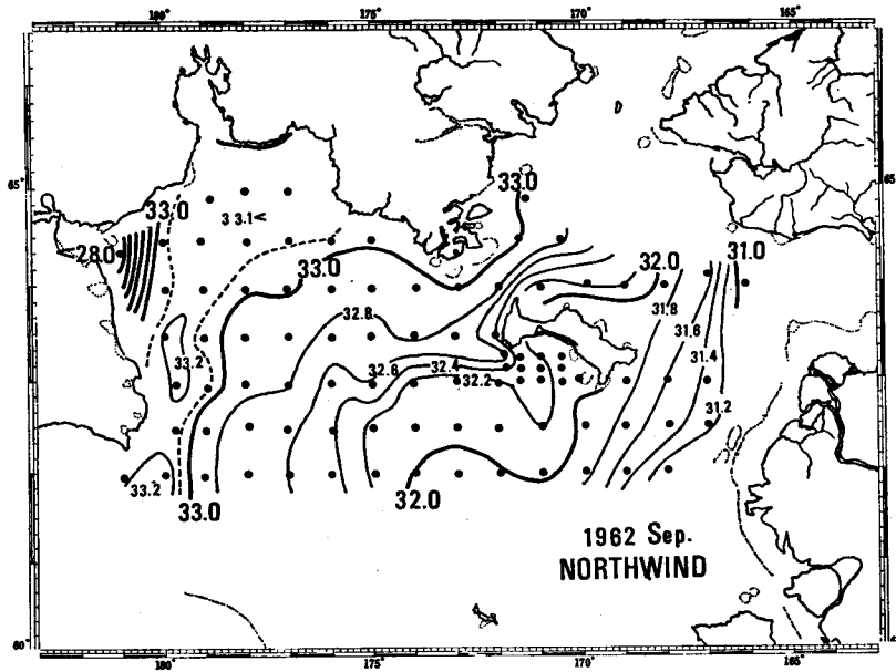
Fig. 28. Salinity distribution at the top of lower layer in the Gulf of Anadur in autumn.
