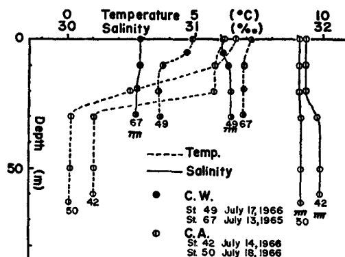
Fig. 38. Typical temperature and salinity structures in C.A. and C.W. regions.
