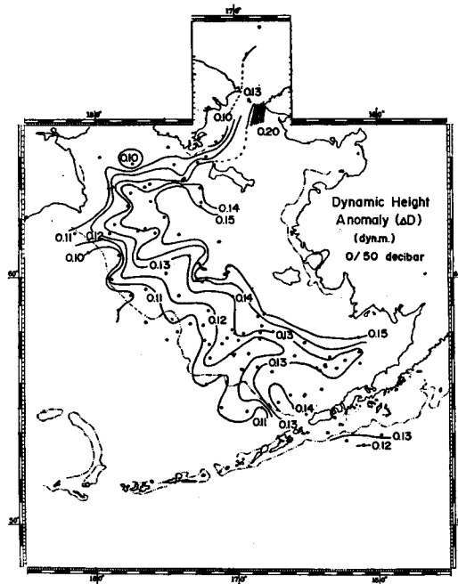
Fig. 11. Dynamic topography, 0/50 decibars.
