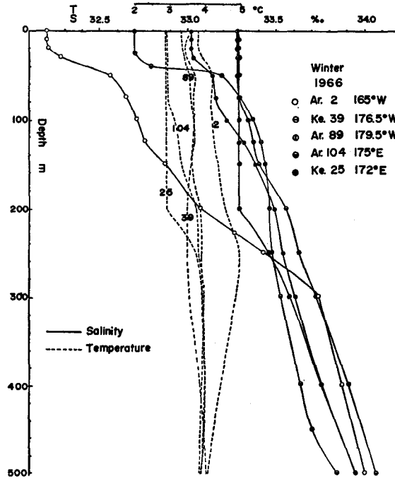
Fig. 9. Vertical distribution of temperature and salinity along the northern boundary of the Alaskan Stream in winter.
