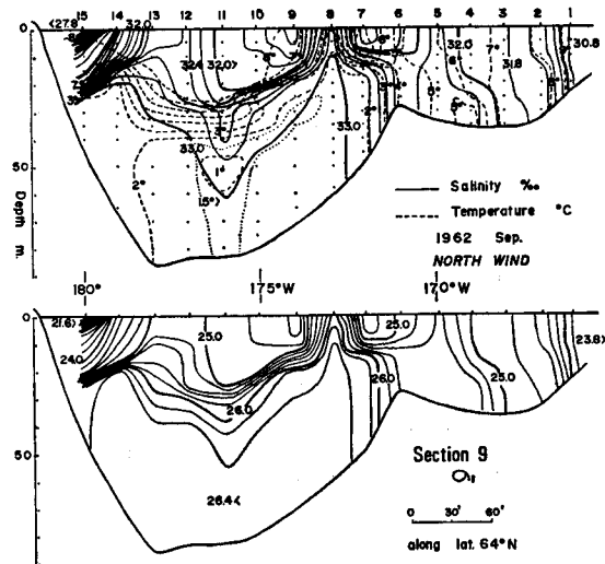
Fig. 36. Vertical sections of temperature, salinity and \sigma_t in the Gulf of Anaduir.
