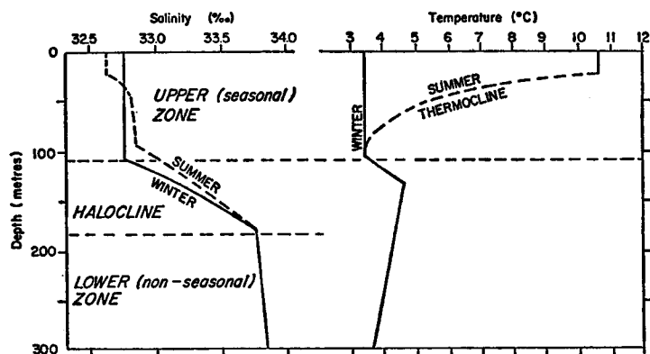
Fig. 1. Schematic structures in the Western Subarctic Pacific Region (Dodimead, 1967).
