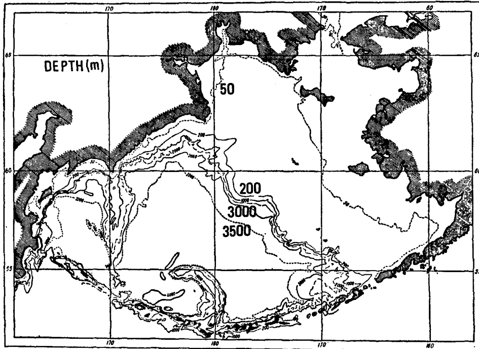
Fig. 4. Sea-bed relief of Bering Sea (Boichenko, from Zenkevitch, 1963).
