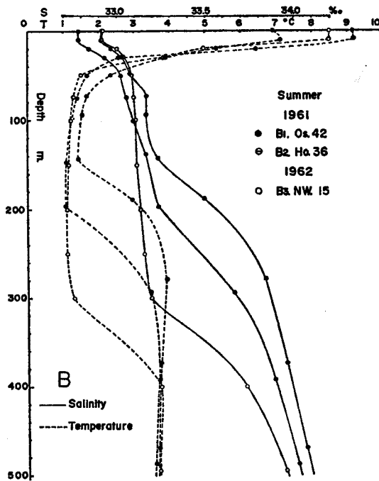
Fig. 19. Salinity and temperature curves of Type B in summer.
