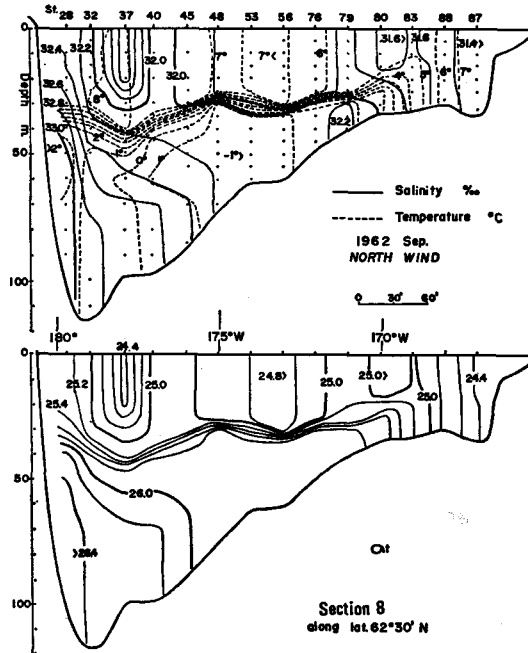
Fig. 35. Vertical sections of temperature, salinity and \sigma_t at the entrance of the Gulf of Anaduir. Locations of Sections are shown in Fig. 29.
