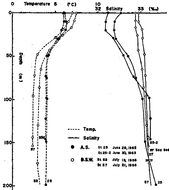
Fig. 37. Typical temperature and salinity structures in A.S. and B.S.W. regions.
