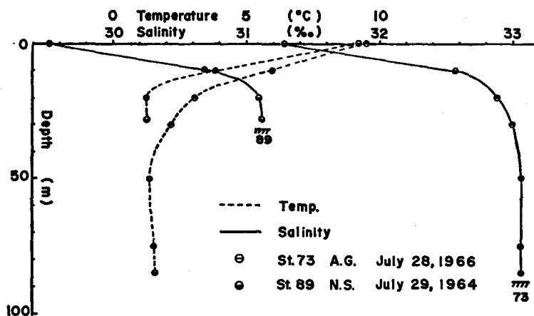
Fig. 39. Typical temperature and salinity structures in A.G. and N.S. regions.
