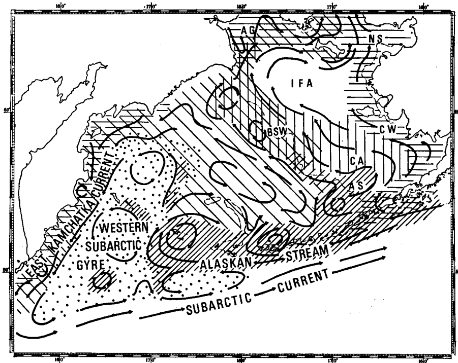
Fig. 46. Schematic representation of flow pattern of shallow waters and extension of type of vertical structure on the shelf.
