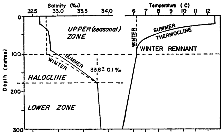
Fig. 2. Schematic structures in the eastern Subarctic Pacific Region (Dodimead & Pickard, 1967).
