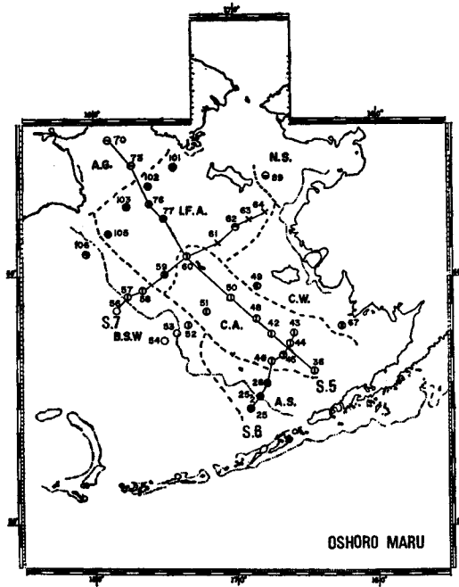
Fig. 41. Location of vertical sections and regions.
