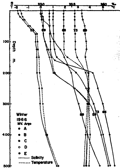
Fig. 22. Salinity and temperature curves of the five Types in winter.
