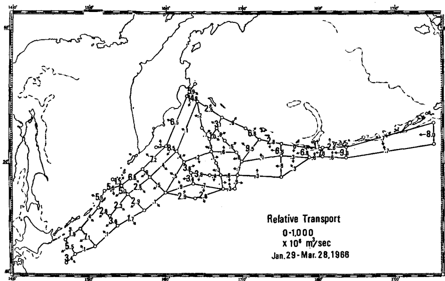
Fig. 5. Relative transport ( \times 10^6 \text{ m}^3/\text{sec} ) in the northwestern Subarctic Region.
