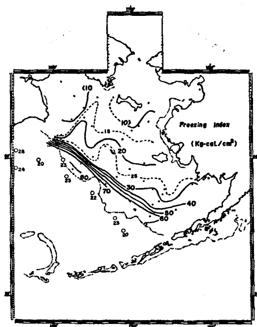
Fig. 43. Freezing indexes for the stations on the shelf and amount of heat given off by the water column in the deep region in winter estimated from the summer observations.
