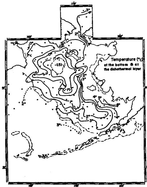
Fig. 31. Temperature distribution at the bottom in summer.
