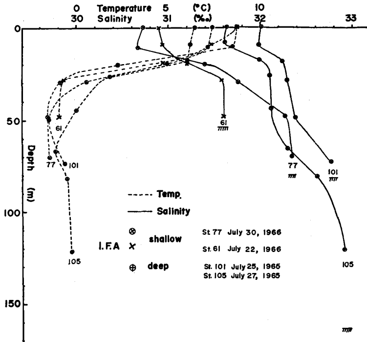
Fig. 40. Typical temperature and salinity structures in I.F.A. region
