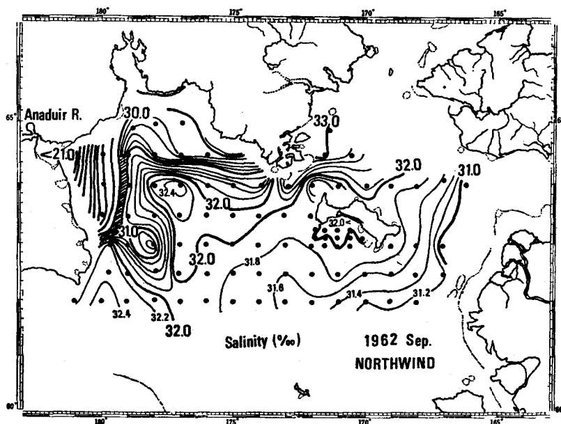
Fig. 26. Horizontal distribution of salinity at the surface in the Gulf of Anaduir in autumn.
