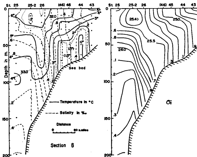
Fig. 33. Vertical sections of temperature, salinity and \sigma_t in the southern part of the shelf.
