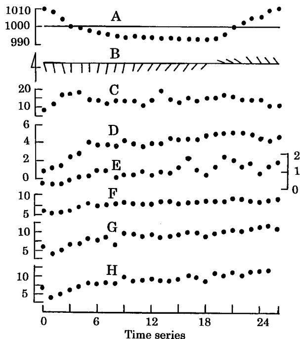
Fig. 2 Time series datas. A: atmospheric pressure (hpa), B: wind direction (degree), C: wind velocity (m/s), D: significant wave height (m), E: maximum elementary wave height (m), F: significant wave period (sec), G: maximum elementary wave period (sec), H: wave period by power spectral (sec)
