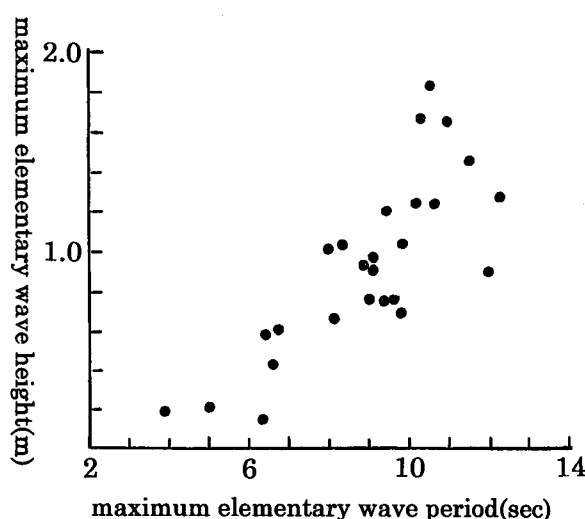
Fig. 4 Relation between wave period ( X axis) and maximum elementary wave height ( Y axis).
