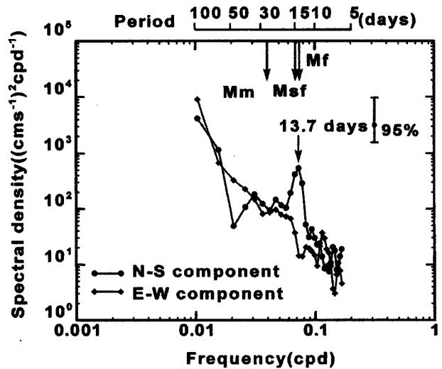
Fig. 10. Power spectral densities of the eastward (diamond) and northward (solid circle) component average flow velocity data at Stns. 5-11 in 48 m depth.
