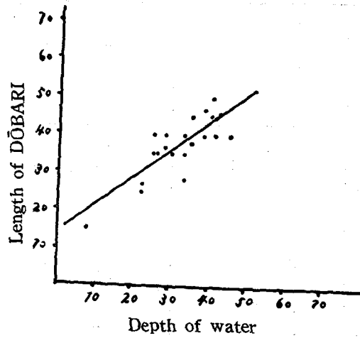
Fig. 4. Length of DÔBARI
