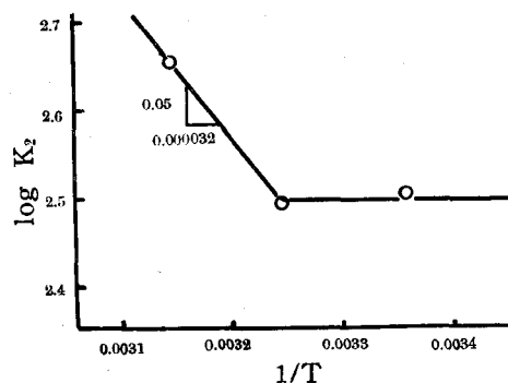
Fig 4. The relation between the values "1/T" and "log K_2 "
