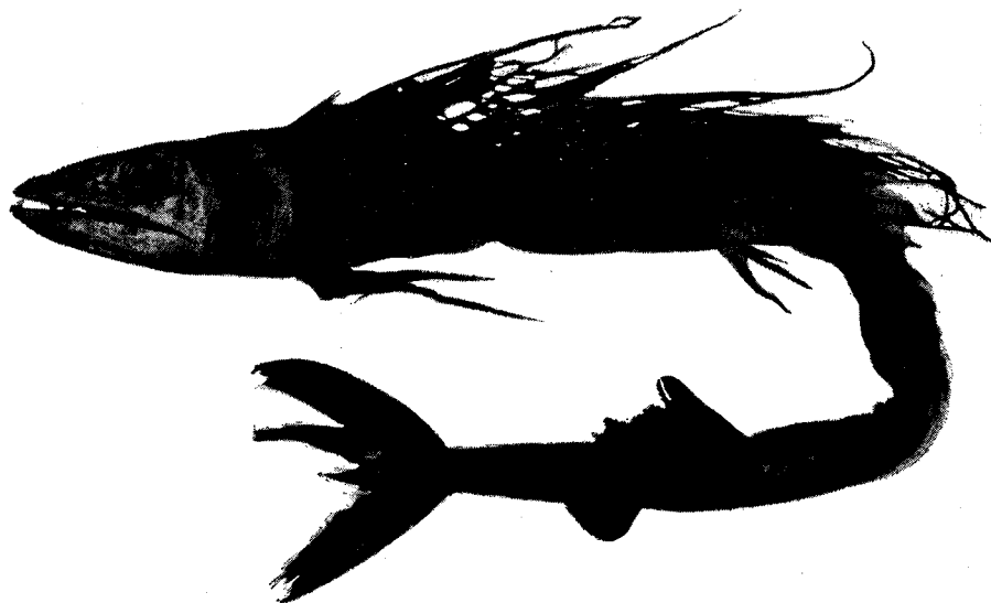
Fig. 4. Alepisaurus ferox (LOWE), 1124mm in total length (Sp. No. 12311)
