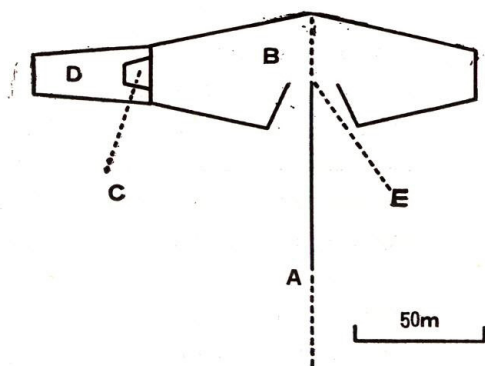
Fig. 3. The scheme of a set-net A : Leading net B : Main net C : Acclivity net D : Pulling net E : Entrance of the main net
