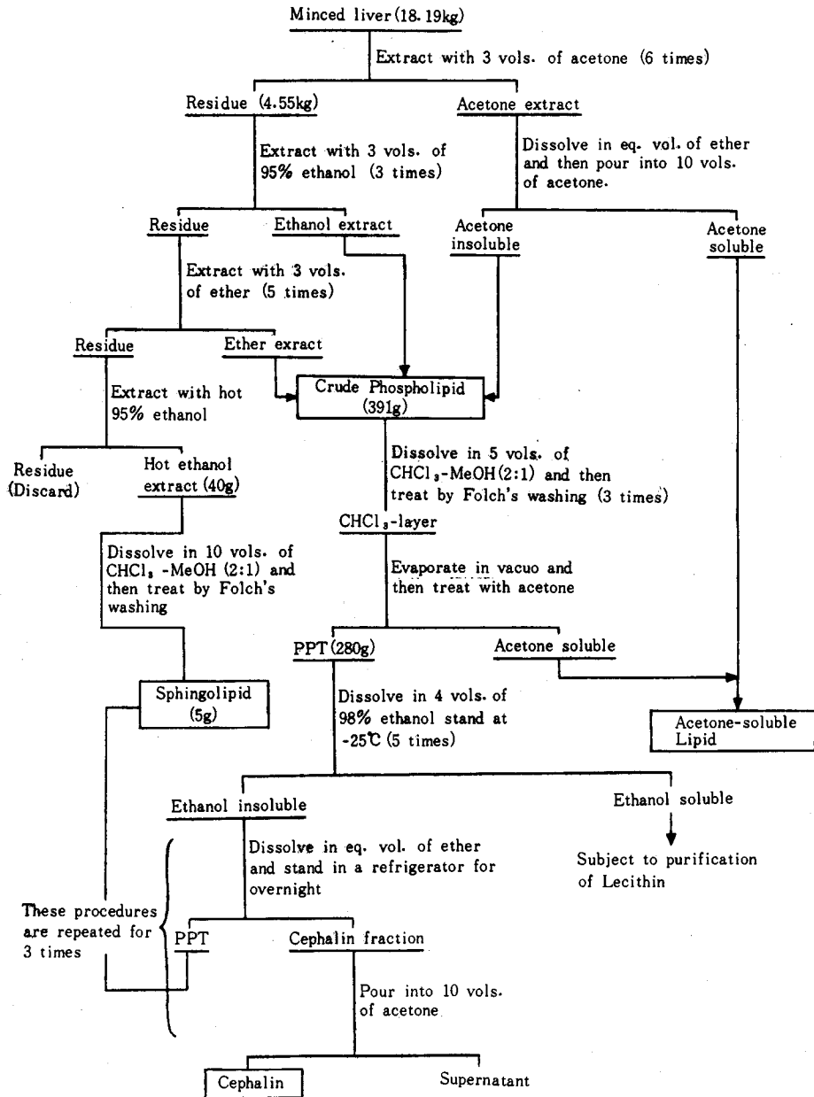
Fig. 1. Preparation of cephalin from salmon liver
