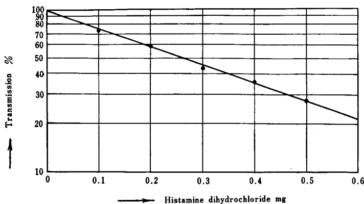
Fig. 1. Calibration curve obtained with histamine dihydrochloride
