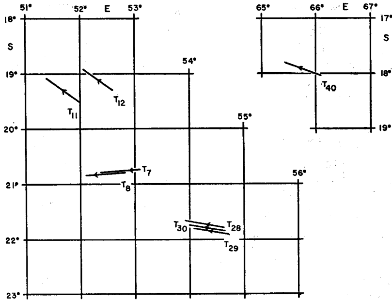
Fig. 1. Positions and directions of long-line fishing set (Taisei-maru, in the eastern area off Madagascar)
