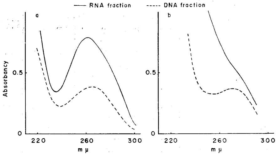
Fig. 2. Ultraviolet absorption spectra of nucleic acid fractions made on ovary a (immature carp); RNA fraction obtained from 1 g of fresh tissue was diluted to 600 ml with 5% HClO 4 . DNA fraction obtained from 1 g of fresh tissue was diluted to 300 ml with 5% HClO 4 . b (mature rainbow trout); RNA fraction and DNA fraction obtained from 1 g of fresh tissue were made up in 50 ml with 5% HClO 4 .
