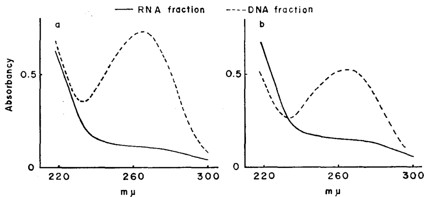
Fig. 1. Ultraviolet absorption spectra of nucleic acid fractions made on blood a (carp); RNA fraction obtained from 1 g of fresh tissue was diluted to 150 ml with 5% \text{HClO}_4 . DNA fraction obtained from 1 g of fresh tissue was diluted to 300 ml with 5% \text{HClO}_4 . b (rainbow trout); RNA fraction obtained from 1 g of fresh tissue was diluted to 187.5 ml with 5% \text{HClO}_4 . DNA fraction obtained from 1 g of fresh tissue was diluted to 375 ml with 5% \text{HClO}_4 .
