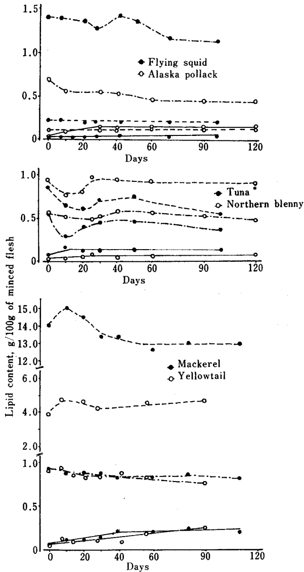
Fig. 1 Changes of lipid content in several stored species of fish at -20^{\circ}\text{C}
