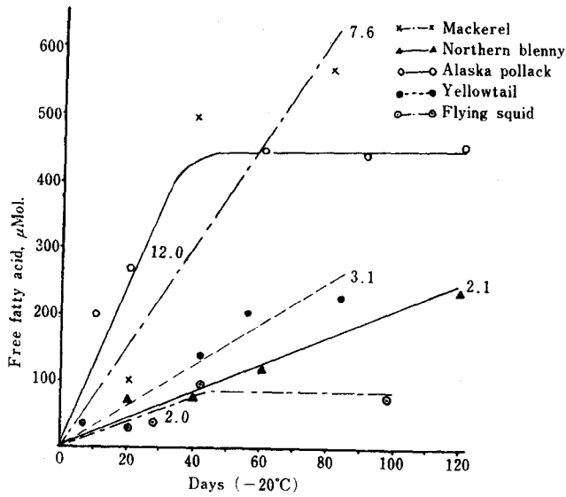
Fig. 2 Developments of free fatty acid during storage at -20^{\circ}\text{C} of various species of fish
