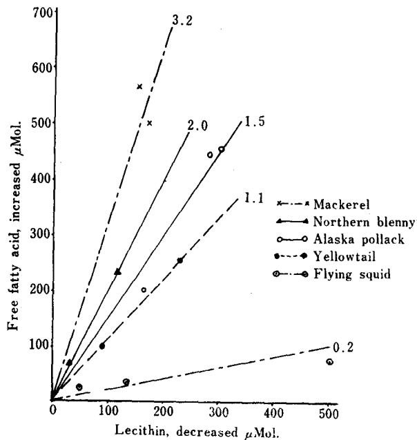
Fig. 3 Relation between decrease of phospholipid (as lecithin) and development of free fatty acid during storage at -20^{\circ}\text{C}
