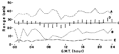
Fig. 7. Range of observed phase difference between point T and point U from 15th of February to 31st of March, 1974.
