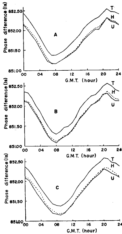
Fig. 4. Average of observed phase difference of A-D pair at points T, H and U. A: From 15th to 28th of February. B: From 1st to 15th of March. C: From 16th to 31st of March.
