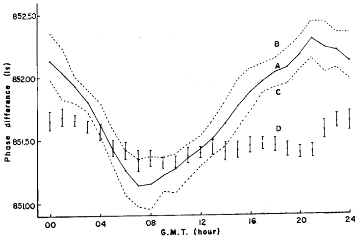
Fig. 3. Observed phase difference of A-D pair at point H from 17th to 28th of February, 1974.
