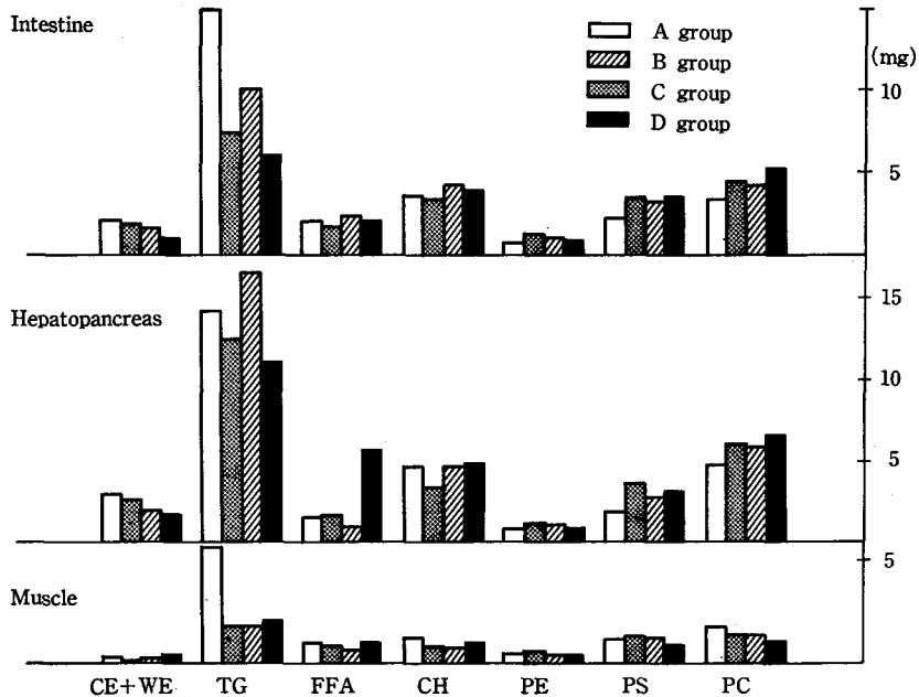
Fig. 2 Lipid compositions of intestine, hepatopancreas and muscle (mg/g organ). WE; Wax ester CE; Cholesterol ester TG; Triglyceride FFA; Free fatty acid CH; Cholesterol PE; Phosphatidyl ethanolamine PS; Phosphatidyl serine PC; Phosphatidyl choline
