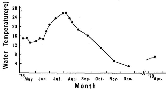
Fig. 2. Monthly changes of water temperature in the waterway from May, 1978 to April, 1979.
