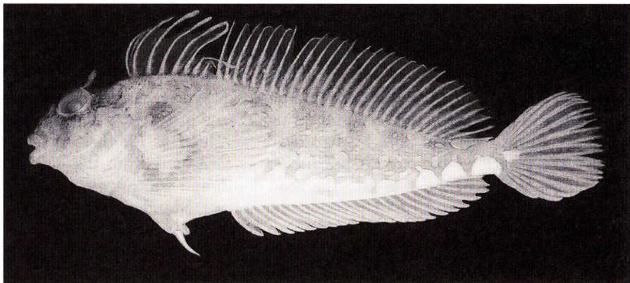
Fig. 1. Archaulus biseriatus Gilbert & Burke, HUMZ 165817, a male, 121.0 mm SL, collected from off Simushir Island, Kuril Archipelago.
