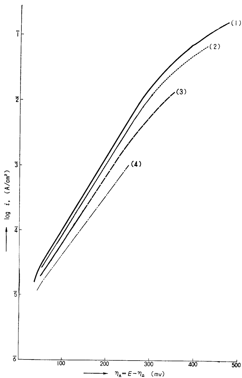
Fig. 11. \log i vs. \eta_A = E - \eta_D (1): 13.68 pH, (2): 12.68 pH, (3): 11.92 pH, (4): 10.72 pH
