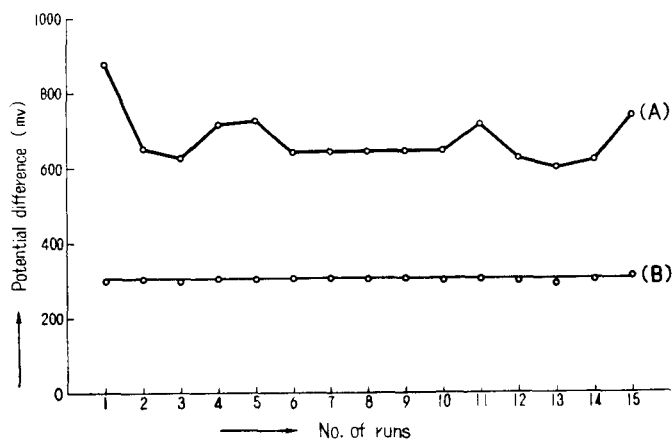
Fig. 10. Potential difference between (R) and (C) at successive switches off, i = 3 \cdot 10^{-3} A/cm 2 , 10.72 pH.
