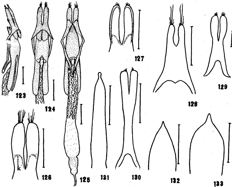
Figs. 123-126. Chlorophorus japonicus . Fig. 123. Lateral view. Fig. 124. Dorsal view. Fig. 125. Ventral view. Fig. 126. Ventral view of lateral lobes. Figs. 127-130. Lateral lobes of Chlorophorus . Fig. 127. Chlorophorus diadema var. inhirsutus . Ventral view. Fig. 128. Ch. notabilis . Dorsal view. Fig. 129. Ch. quinquefasciatus . Dorsal view. Fig. 130. Ch. annularis . Dorsal view. Figs. 131-133. Median lobe of Chlorophorus . All ventral view. Fig. 131. Chlorophorus annularis . Fig. 132. Ch. notabilis . Fig. 133. Ch. quinquefasciatus .
