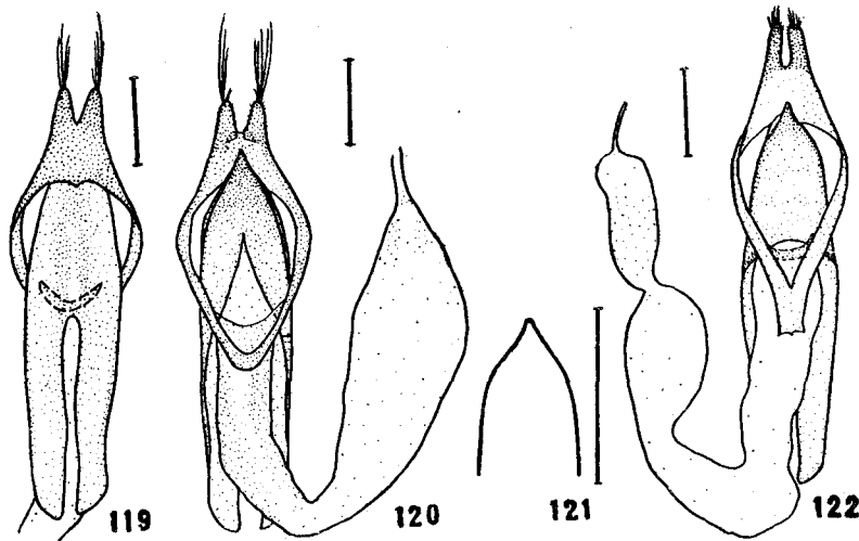
Figs. 119-120. Cyrtoclytus caproides . Fig. 119. Dorsal view. Fig. 120. Ventral view. Fig. 121. Apical part of median lobe of Brachyclytus singularis . Ventral view. Fig. 122. Plagionotus pulcher . Ventral view.
