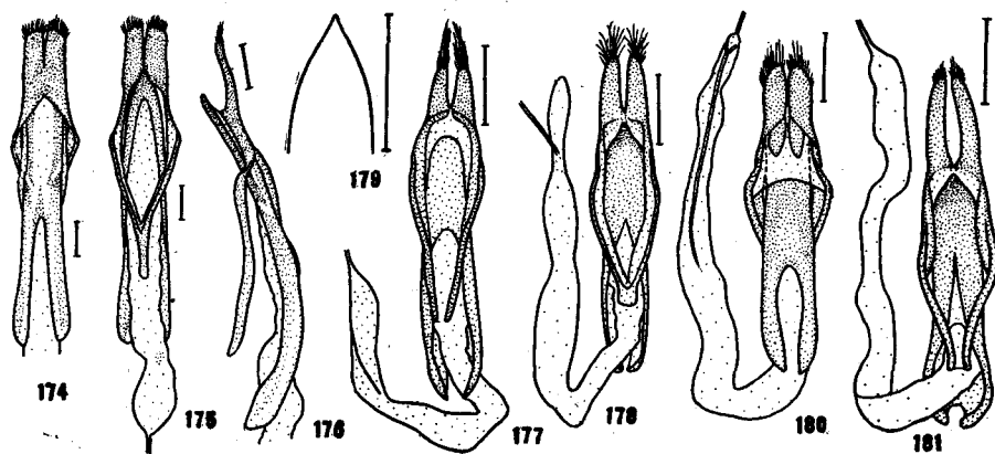
Figs. 174-176. Apalimna liturata . Fig. 174. Dorsal view. Fig. 175. Ventral view. Fig. 176. Lateral view. Fig. 177. Jezohammus nubilus . Ventral view. Fig. 178. Pterolophia jugosa . Ventral view. Fig. 179. Apical part of median lobe of Pterolophia rigida . Ventral view. Fig. 180. Asaperda agapanthina . Dorsal view. Fig. 181. Rhopaloscelis unifasciatus . Ventral view.
