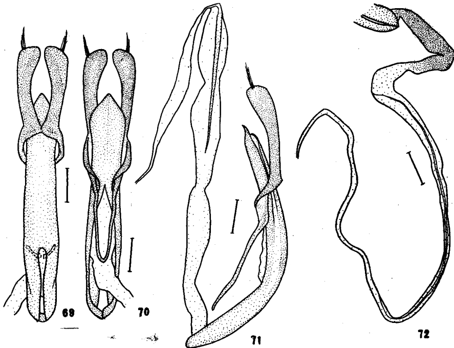
Figs. 69-72. Strangalia (Strangalia) arcuata f. mimica . Fig. 69. Dorsal view. Fig. 70. Ventral view. Fig. 71. Lateral view. Fig. 72. Internal sac of Strangalia (Strangalia) aethiops .
