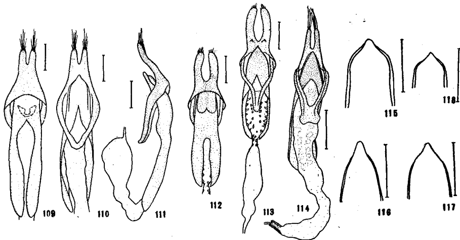
Figs. 109-111. Xylotrechus chinensis . Fig. 109. Dorsal view. Fig. 110. Ventral view. Fig. 111. Lateral view. Figs. 112-113. Clytus auripilis . Fig. 112. Dorsal view. Fig. 113. Ventral view. Fig. 114. Clytus melaenus . Ventral view. Figs. 115-117. Apical part of median lobe of Xylotrechus . All ventral view. Fig. 115. Xylotrechus chinensis . Fig. 116. X. clarinus . Fig. 117. X. cuneipennis . Fig. 118. X. pyrrhoderus .
