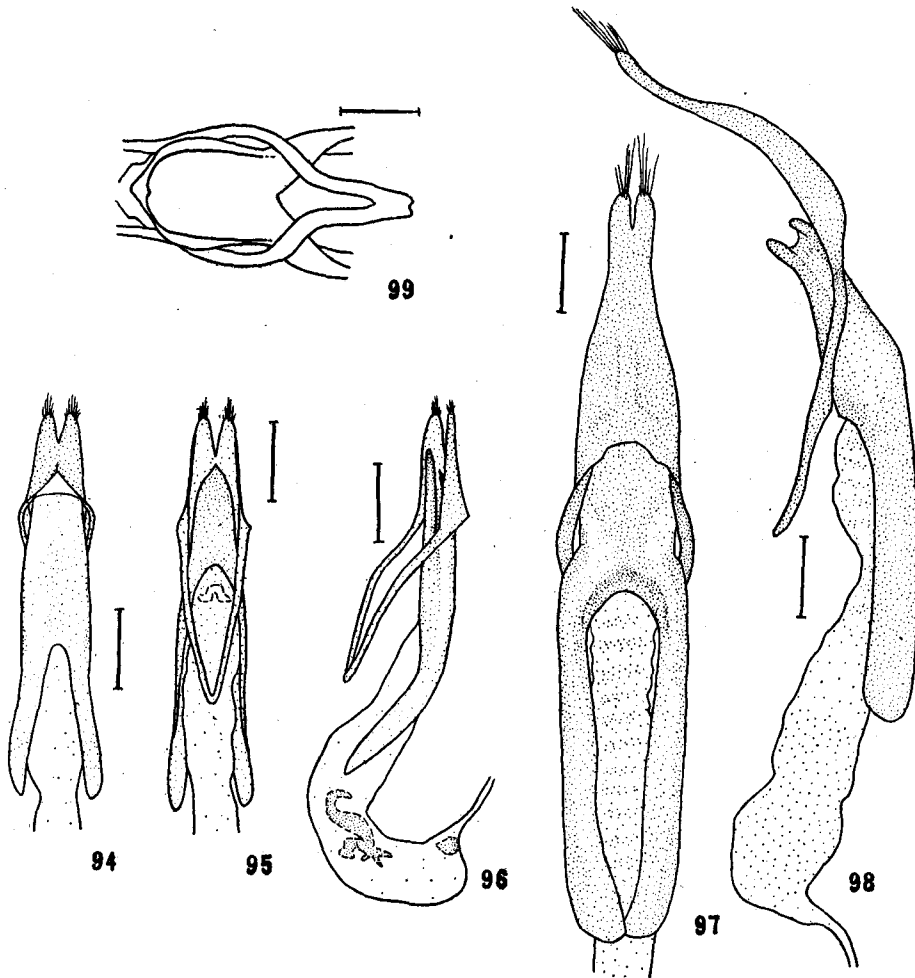
Figs. 94-96. Leontium viride . Fig. 94. Dorsal view. Fig. 95. Ventral view. Fig. 96. Lateral view. Figs. 97-99. Rosalia (Rosalia) batesi . Fig. 97. Dorsal view. Fig. 98. Lateral view. Fig. 99. Ventral view of median lobe and ringed part.
