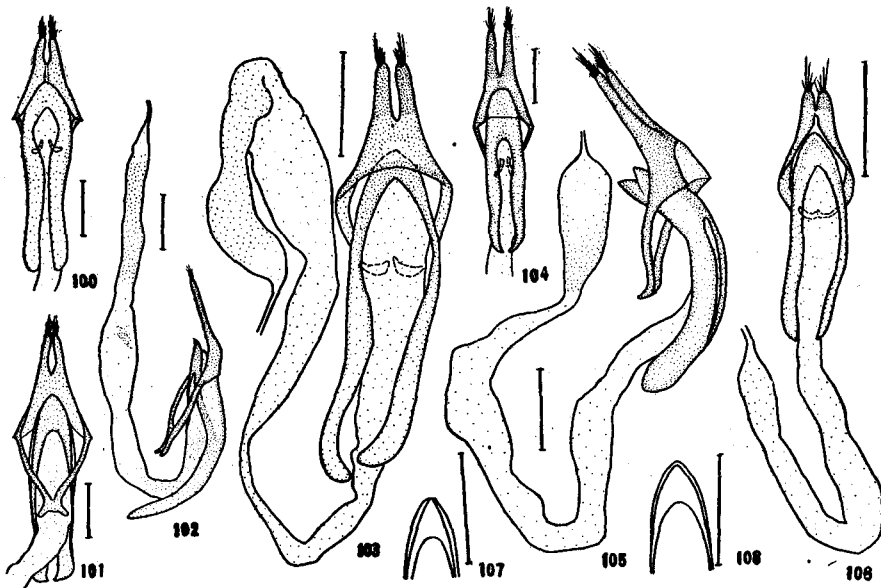
Figs. 100-102. Rhopalopus ( Prorrhopalopus ) signaticollis . Fig. 100. Dorsal view. Fig. 101. Ventral view. Fig. 102. Lateral view. Fig. 103. Semanotus rufipennis . Dorsal view. Figs. 104-105. Callidium ( Callidium ) violaceum . Fig. 104. Dorsal view. Fig. 105. Lateral view. Figs. 106-107. Phymatodes ( Paraphymatodes ) albicinctus . Fig. 106. Dorsal view. Fig. 107. Ventral view of median lobe. Fig. 108. Median lobe of Phymatodes ( Poecilium ) maaki . Ventral view.
