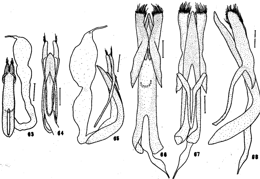
Fig. 63. Strangalomorpha tenuis . Dorsal view. Figs. 64-65. Eustrangalis distenioides . Fig. 64. Ventral view. Fig. 65. Lateral view. Figs. 66-68. Oedecnema dubia . Fig. 66. Dorsal view. Fig. 67. Ventral view. Fig. 68. Lateral view.
