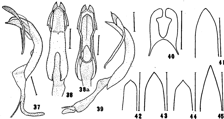
Fig. 37. Pidonia (Pidonia) maculithorax . Lateral view. Figs. 38-39. Pidonia (Pseudopidonia) grallatrix . Fig. 38. Dorsal view. Fig. 38a. Ventral view. Fig. 39. Lateral view. Fig. 40. Lateral lobes of Pidonia (Pseudopidonia) debilis . Dorsal view. Figs. 41-45. Apical part of median lobe of the subgenus Pseudopidonia . All ventral view. Fig. 41. Pidonia (Pseudopidonia) grallatrix . Fig. 42. P. (Ps.) amentata . Fig. 43. P. (Ps.) debilis . Fig. 44. P. (Ps.) insuturata . Fig. 45. P. (Ps.) signifera .
