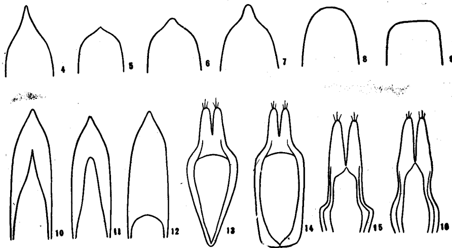
Figs. 4-9. Types of apical part of median lobe (Schematic). All ventral view. Fig. 4. Sharply pointed. Fig. 5. Bluntly pointed. Fig. 6. Weakly projected. Fig. 7. Strongly projected. Fig. 8. Rounded. Fig. 9. Truncated. Figs. 10-12. Types of median foramen. All ventral view. Figs. 10-11. Elongated. Fig. 12. Not elongated. Figs. 13-14. Types of ringed part. Both ventral view. Fig. 13. Converging. Fig. 14. Nearly parallel. Figs. 15-16. Geniculation and constriction of ringed part. Both ventral view. Fig. 15. Geniculated. Fig. 16. Constricted.
