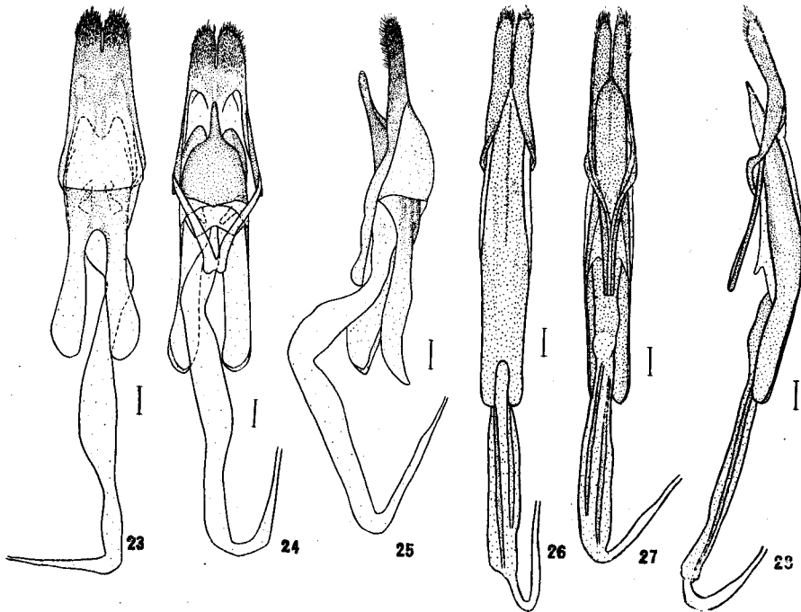
Figs. 23-25. Prionus insularis . Fig. 23. Dorsal view. Fig. 24. Ventral view. Fig. 25. Lateral view. Figs. 26-28. Distenia gracilis . Fig. 26. Dorsal view. Fig. 27. Ventral view. Fig. 28. Lateral view.
