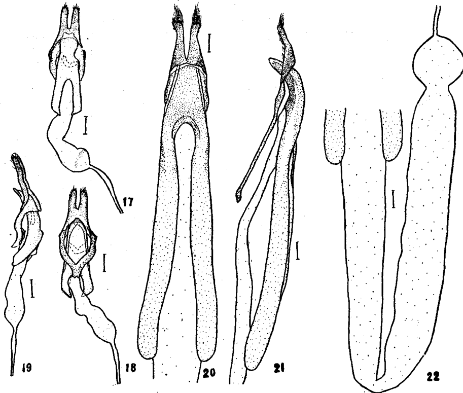
Figs. 17-19. Spondylis buprestoides . Fig. 17. Dorsal view. Fig. 18. Ventral view. Fig. 19. Lateral view. Figs. 20-22. Megopis (Aegosoma) sinica sinica . Fig. 20. Dorsal view. Fig. 21. Lateral view. Fig. 22. Internal sac.
