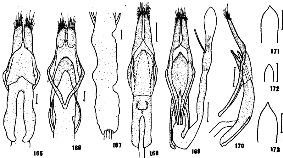
Figs. 165-167. Apriona germari . Fig. 165. Dorsal view. Fig. 166. Ventral view. Fig. 167. Internal sac. Figs. 168-171. Mesosa myops var. japonica . Fig. 168. Dorsal view. Fig. 169. Ventral view. Fig. 170. Lateral view. Fig. 171. Ventral view of apical part of median lobe. Figs. 172-173. Apical part of median lobe of Mesosa . Both ventral view. Fig. 172. Mesosa hirsuta . Fig. 173. M. longipennis .
