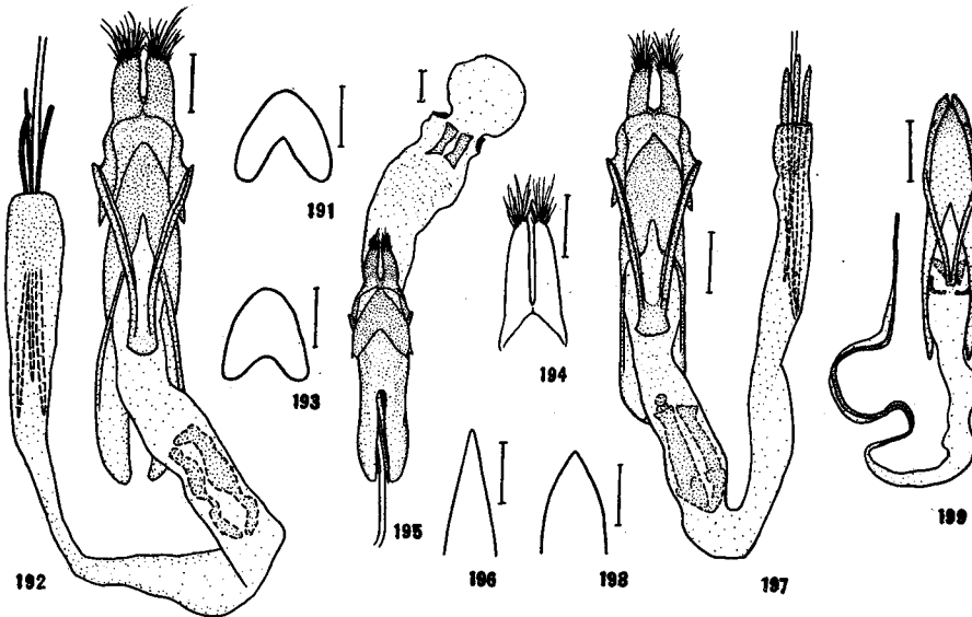
Fig. 191. Basal-piece of Saperda octomaculata . Dorsal view. Figs. 192-193. Eutetrappa ocelota . Fig. 192. Ventral view. Fig. 193. Dorsal view of basal-piece. Fig. 194. Lateral lobes of Eutetrappa sedecimpunctata . Dorsal view. Fig. 195. Cagosima sanguinolenta . Dorsal view. Fig. 196. Apical part of median lobe of Glenea (Glenea) relicta . Ventral view. Fig. 197. Paraglenea fortunei . Ventral view. Fig. 198. Apical part of median lobe of Paraglenea chrysochloris . Ventral view. Fig. 199. Chreonema fortunei . Ventral view.
