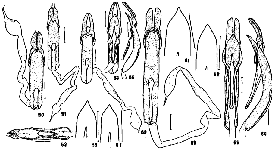
Fig. 50. Leptura (Anoploderomorpha) cyanea . Dorsal view. Figs. 51-52. Leptura (Kanekoa) azumensis . Fig. 51. Dorsal view. Fig. 52. Ventral view. Figs. 53-56. Leptura (Leptura) scotodes . Fig. 53. Dorsal view. Fig. 54. Ventral view. Fig. 55. Lateral view. Fig. 56. Ventral view of apical part of median lobe. Fig. 57. Apical part of median lobe of Leptura (Leptura) sequensi . Ventral view. Figs. 58-61. Leptura (Leptura) succedanea . Fig. 58. Dorsal view. Fig. 59. Ventral view. Fig. 60. Lateral view. Fig. 61. Ventral view of apical part of median lobe. Fig. 62. Apical part of median lobe of Leptura (Leptura) variicornis . Ventral view.
