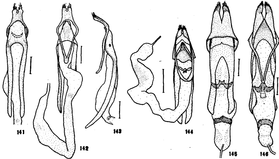
Figs. 141-143. Paraclytus exultus . Fig. 141. Dorsal view. Fig. 142. Ventral view. Fig. 143. Lateral view. Fig. 144. Dere thoracica . Ventral view. Figs. 145-146. Purpuricenus spectabilis . Fig. 145. Dorsal view. Fig. 146. Ventral view.
