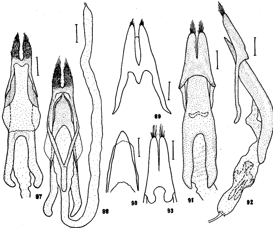
Figs. 87-88. Criocephalus (Megasemum) quadricostulatum . Fig. 87. Dorsal view. Fig. 88. Ventral view. Figs. 89-90. Mallambyx raddei . Fig. 89. Dorsal view of lateral lobes. Fig. 90. Ventral view of median lobe. Figs. 91-92. Aromia (Aromia) moschata var. orientalis . Fig. 91. Dorsal view. Fig. 92. Lateral view. Fig. 93. Lateral lobes of Chloridolum (Parachloridolum) thaliodes . Dorsal view.
