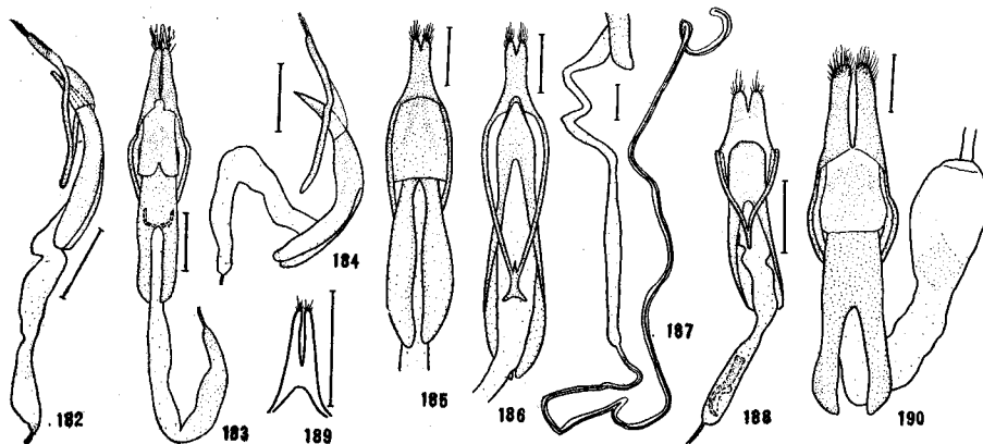
Fig. 182. Terinaea atrofusca . Lateral view. Fig. 183. Sydonia divaricata . Dorsal view. Fig. 184. Pogonocherus (Pogonocherus) seminiveus . Lateral view. Figs. 185-187. Acanthocinus (Acanthocinus) griseus . Fig. 185. Dorsal view. Fig. 186. Ventral view. Fig. 187. Internal sac and ejaculatory duct. Fig. 188. Exocentrus guttulatus . Ventral view. Fig. 189. Lateral lobes of Exocentrus fasciolatus . Dorsal view. Fig. 190. Agapanthia daurica . Dorsal view.
