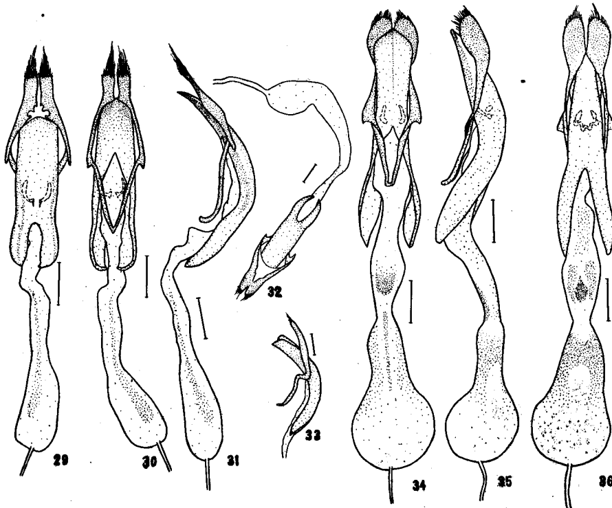
Figs. 29-31. Rhagium (Hargium) inquisitor japonicum . Fig. 29. Dorsal view. Fig. 30. Ventral view. Fig. 31. Lateral view. Figs. 32-33. Stenocorus coeruleipennis . Fig. 32. Dorsal view. Fig. 33. Lateral view. Figs. 34-36. Gaurotus (Paragaurotus) doris . Fig. 34. Ventral view. Fig. 35. Lateral view. Fig. 36. Dorsal view.
