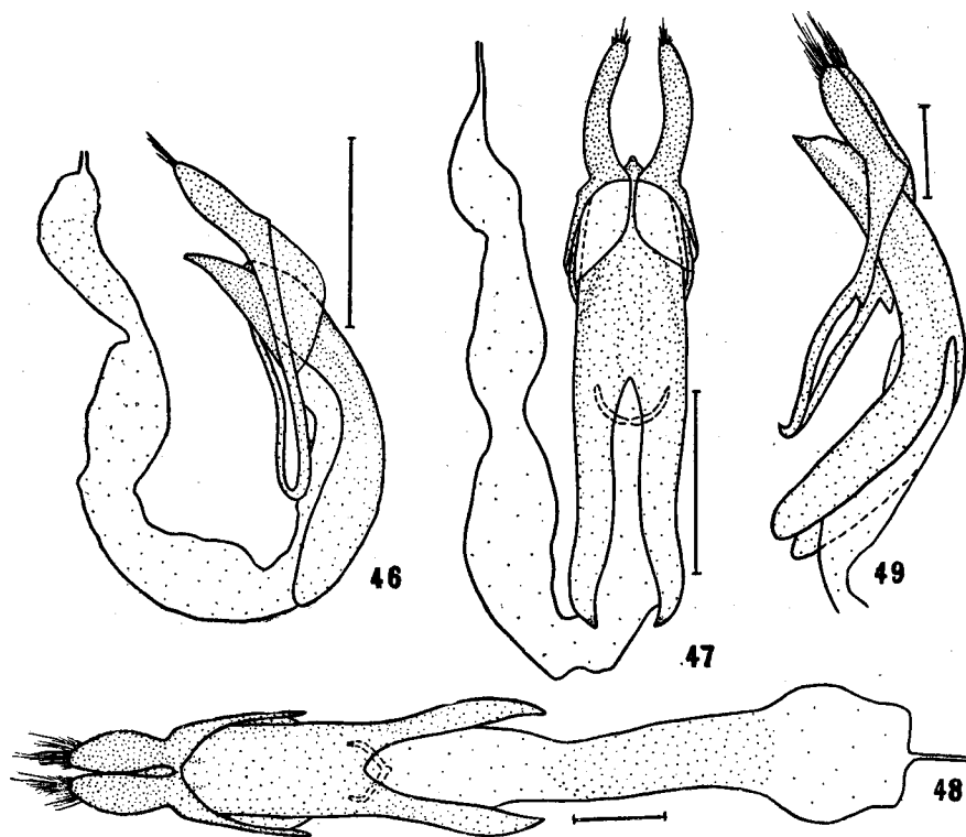
Fig. 46. Grammoptera elegantula . Lateral view. Fig. 47. Alosterna tabacicolor . Dorsal view. Figs. 48-49. Judolia (Judolia) cometes . Fig. 48. Dorsal view. Fig. 49. Lateral view.
