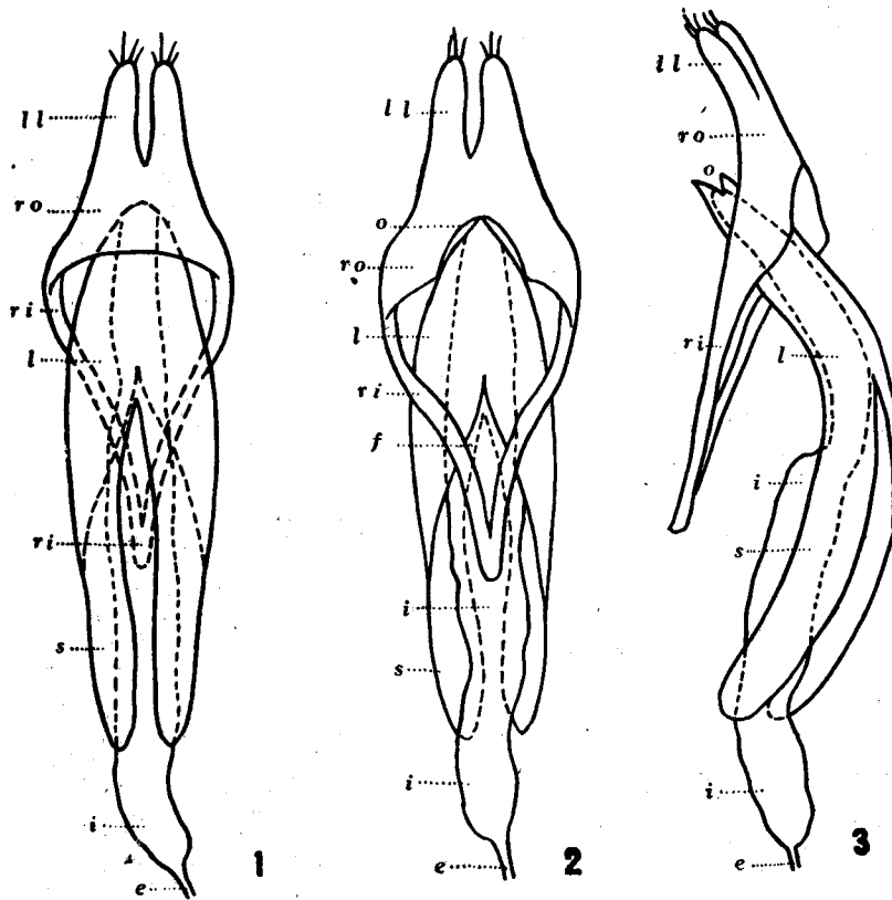
Figs. 1-3. A type of male genitalia of cerambycid beetles, showing the technical terms (Schematic). Fig. 1. Dorsal view. Fig. 2. Ventral view. Fig. 3. Lateral view. e. Ejaculatory duct. f. Median foramen. i. Internal sac. 1. Median lobe. ll. Lateral lobes. o. Median orifice. ri. Ringed part. ro. Roof. s. Median struts.
