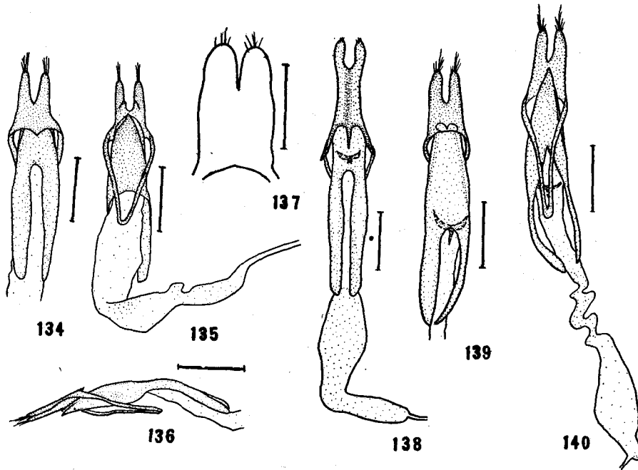
Figs. 134-136. Raphuma xenisca . Fig. 134. Dorsal view. Fig. 135. Ventral view. Fig. 136. Lateral view. Fig. 137. Lateral lobes of Aglaophis colobothoides . Dorsal view. Fig. 138. Demodex transilis . Dorsal view. Figs. 139-140. Anaglyptus niponensis . Fig. 139. Dorsal view. Fig. 140. Ventral view.
