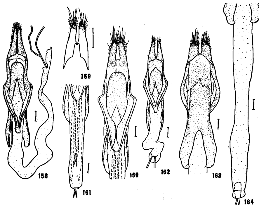
Fig. 158. Dihammus luxuriosus . Ventral view. Fig. 159. Lateral lobes of Dihammus fraudator . Dorsal view. Figs. 160-161. Melanauster chinensis var. macularius . Fig. 160. Ventral view. Fig. 161. Internal sac. Fig. 162. Eupromus ruber . Ventral view. Figs. 163-164. Batocera (Batocera) lineolata . Fig. 163. Dorsal view. Fig. 164. Internal sac.
