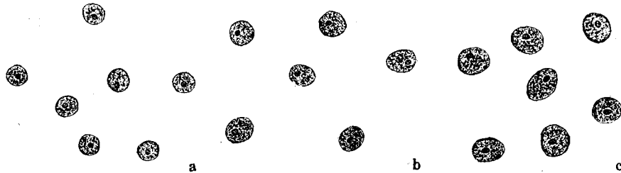
Fig. 1. Morphological comparison of nuclei. ( 10 \times 100 ). a, Carp. b, F_1 . c, Funa.
