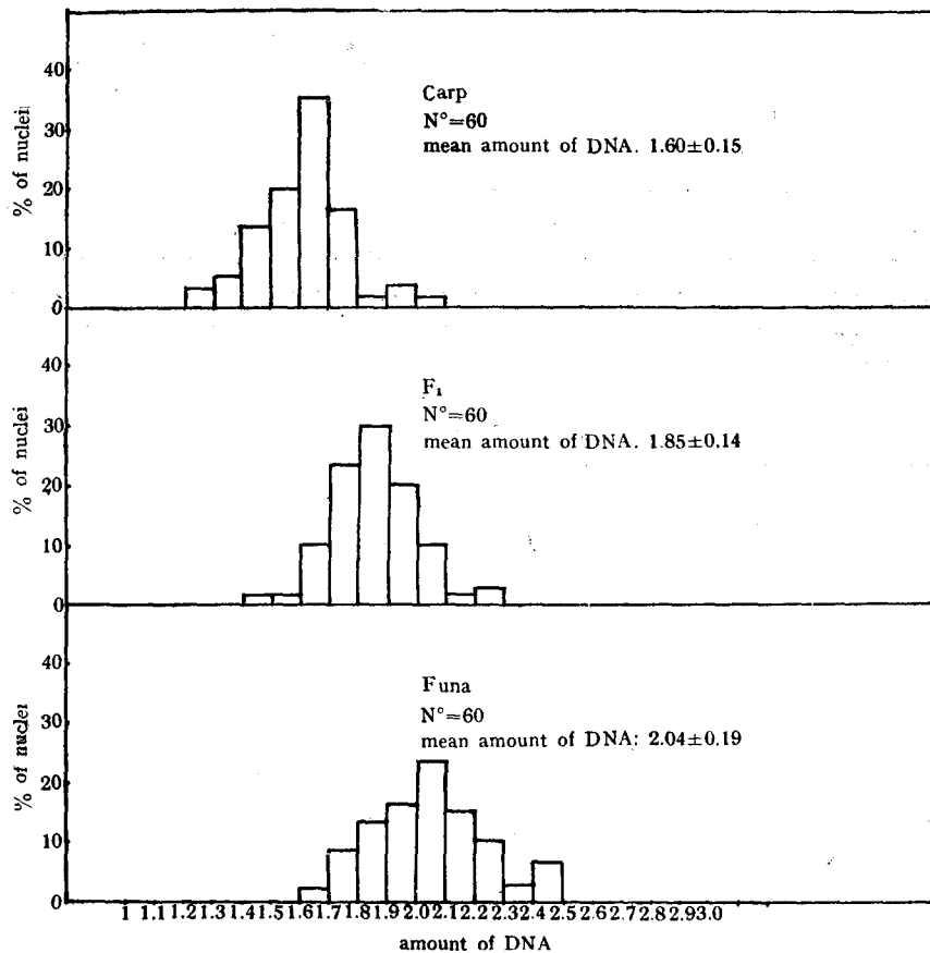
Fig. 2. Comparison of the amount of DNA (microspectrophotometry) in individual nuclei of the Carp, the Funa and their hybrid. N°=number of nuclei measured.
