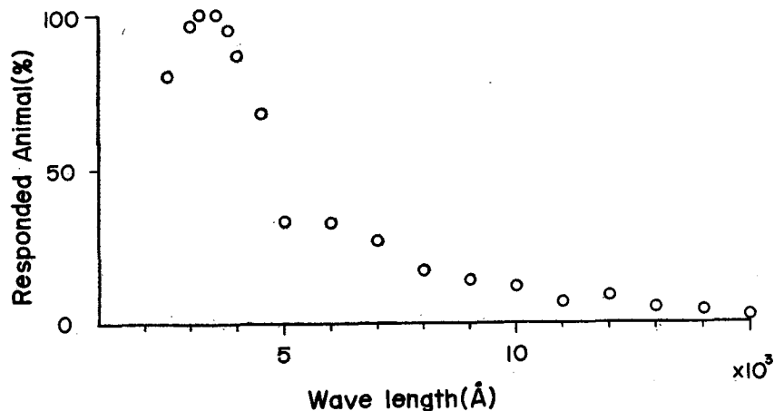
Fig. 6. Spectrum sensitivity curve of Paramecium . Ordinate: % of animals responding. Abscissa: wave length in Å. The radiation energy of monochromatic light was kept constant in each wave length.
