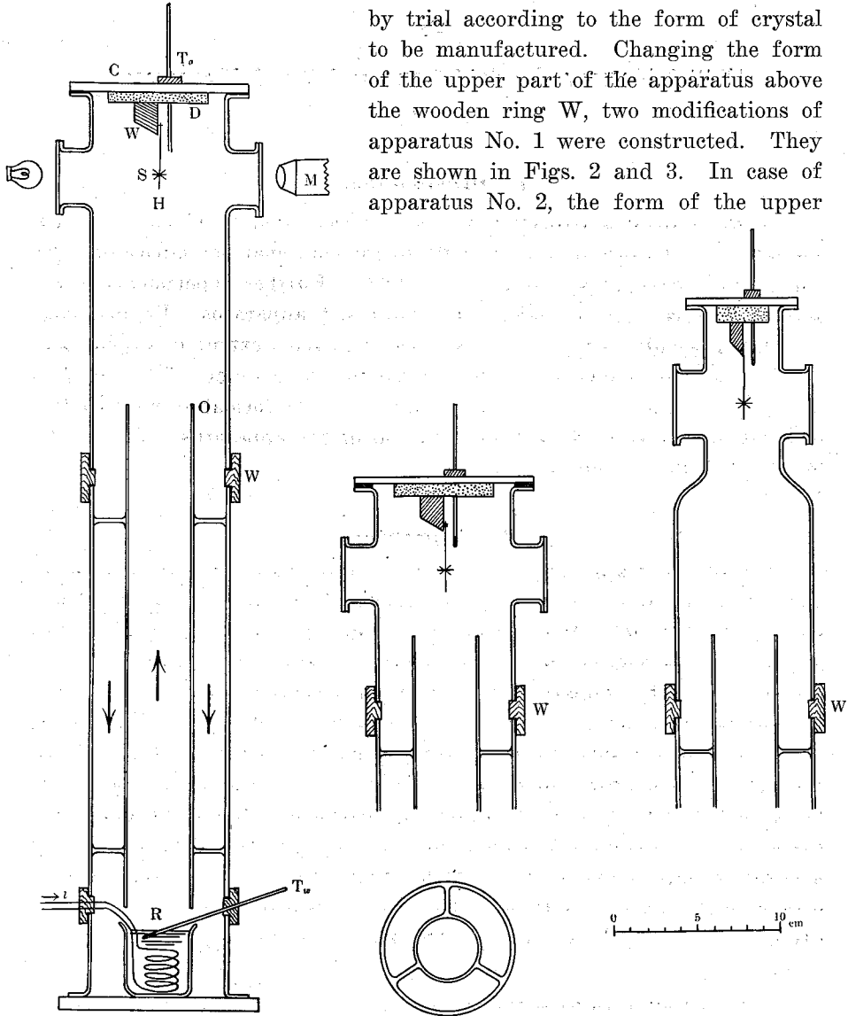
Fig. 1. Apparatus No. 1.
