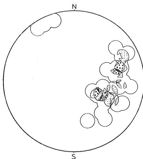
Fig. 12 Lineation diagram of Oshirabetsu dome.
