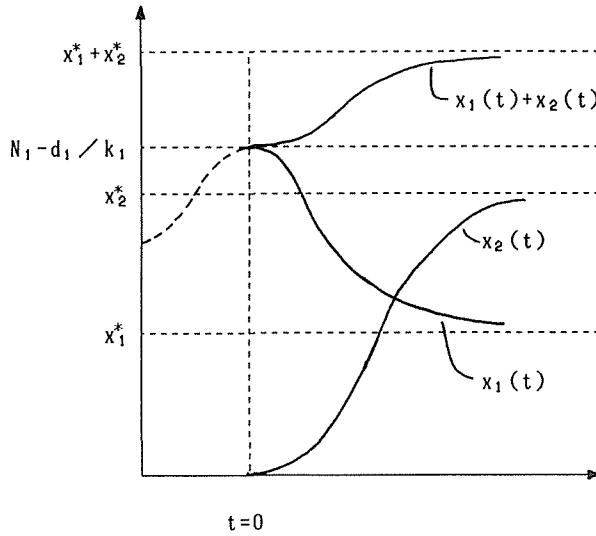
Figure. 11 Regional Population ( 0 < \beta < 1 ) Note : x_1^* = \{N_1 - d_1 / k_1 - \beta(N_2 - d_2 / k_2)\} / (1 - \beta^2) x_2^* = \{N_2 - d_2 / k_2 - \beta(N_1 - d_1 / k_1)\} / (1 - \beta^2)
