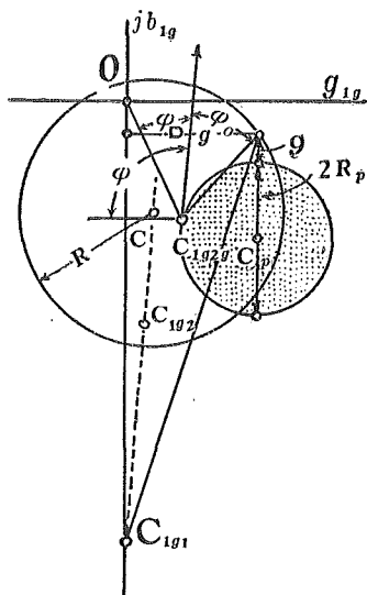
Fig. 2 Circle to keep the terminal voltages constant. Inside the shaded circle to act as a motor.
