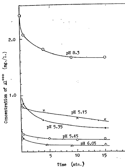
Fig. 7. Polymerization of Al ion at 25°C. Initial concn. of \text{Al}^{\text{III}} , 2.42 mg./l.; pH adjusted with NaOH; \text{AlCl}_3 was used.
