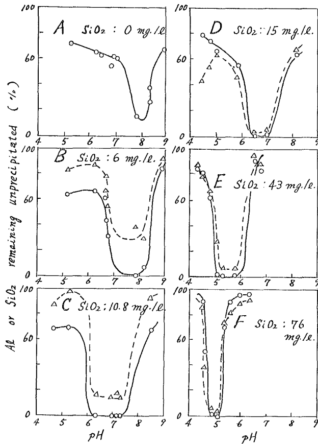
Fig. 14. Effect of varying amount of colloidal \text{SiO}_2 (specific surface area, 1100 sq. m./g.) ○ Al, △ \text{SiO}_2 in the solution filtered 10 min. after pH adjustment.
