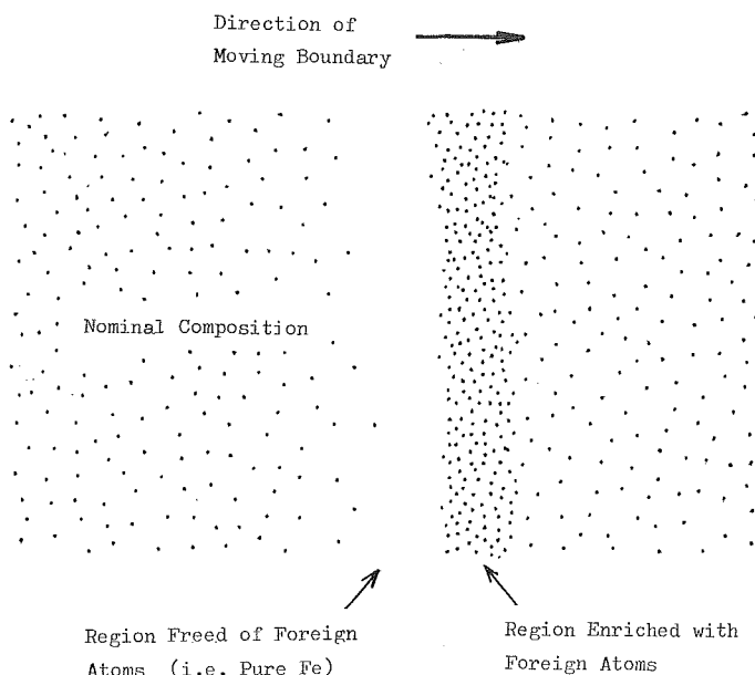
Fig. 7. Regions of deviated compositions from nominal one afterward and forward of moving boundary (Schematic)
