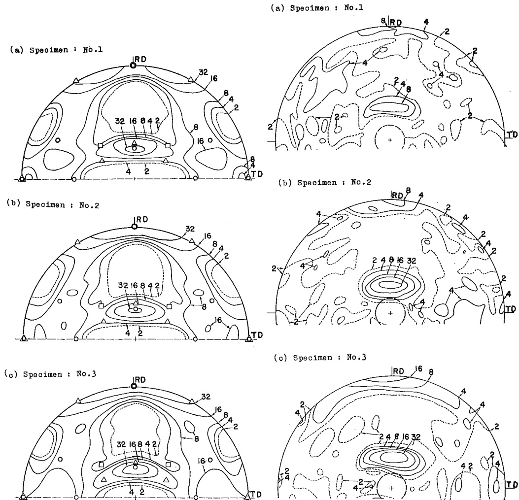
Fig. 1. (110)-pole figures of cold rolled 3.17% Al-Fe alloy sheets by 70% to 3.5 mm in thickness. Symbols \triangle , \circ and \square indicate (111) [11\bar{2}] , (112) [1\bar{1}2] and (100) [011] poles respectively.
