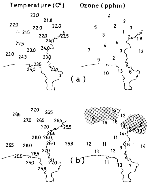
Fig. 8. Horizontal distribution of ozone concentration and temperature at the altitude of 300 m on July 19, 1973. Fig. (a) and (b) are observed at 0935-1106 and 1327-1406 JST respectively.
