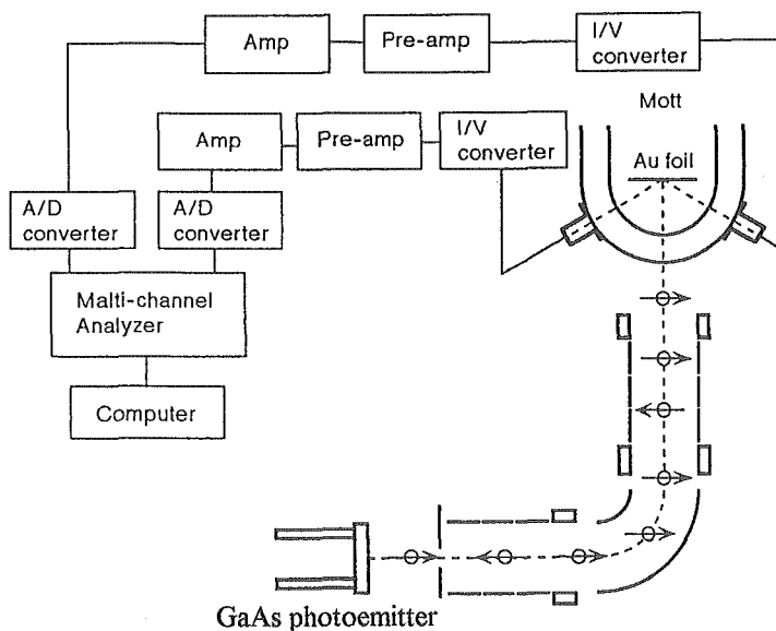
Fig. 6 Schematic diagram of the static lens system and the electron counting system.
