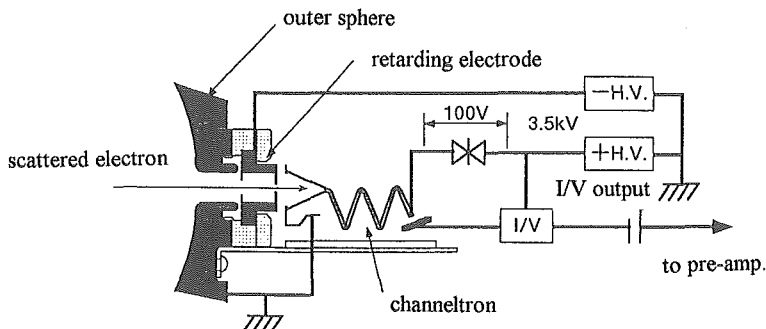
Fig. 5 Schematic diagram of the electron detection system.
