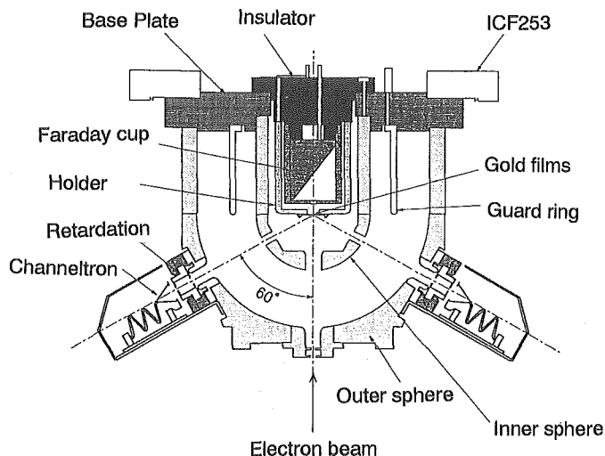
Fig. 3 Schematic diagram of the Mott polarimeter.
