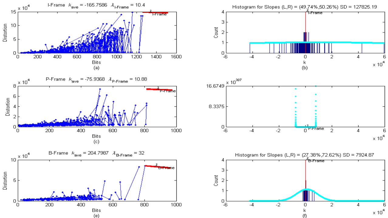
Fig. 7. Visualizing the performances of a DCT-like kernel IK(1,2,1) and an IST Kernel for Sequence Tempete at QP = 24 . Note that the \lambda 's for kernel selections are shown using red color. (a) Line segments of all macroblock of I-Frame. (b) The distribution of the slopes of line segments of I-Frame. (c) Line segments of all macroblock of P-Frame. (d) The distribution of the slopes of line segments of P-Frame. (e) Line segments of all macroblock of B-Frame. (f) The distribution of the slopes of line segments of B-Frame.
